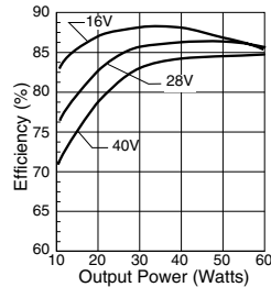
MFL2812S & MFL2812D Efficiency FIGURE 5
