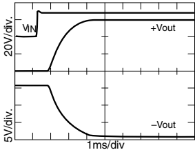
MFL2815D Turn On Response
