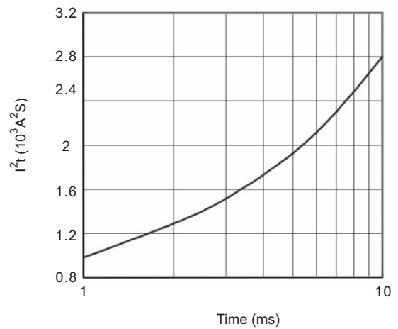
Fig.6 I²t characteristic
