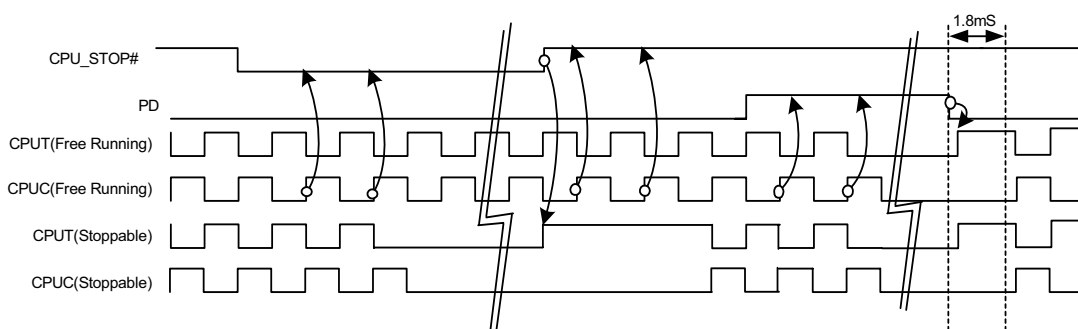
Figure 8. CPU_STOP# = Hi-Z, CPU_PD = Hi-Z
