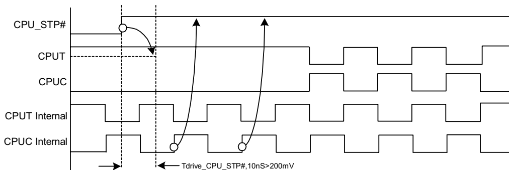
Figure 6. CPU_STP# Deassertion Waveform
