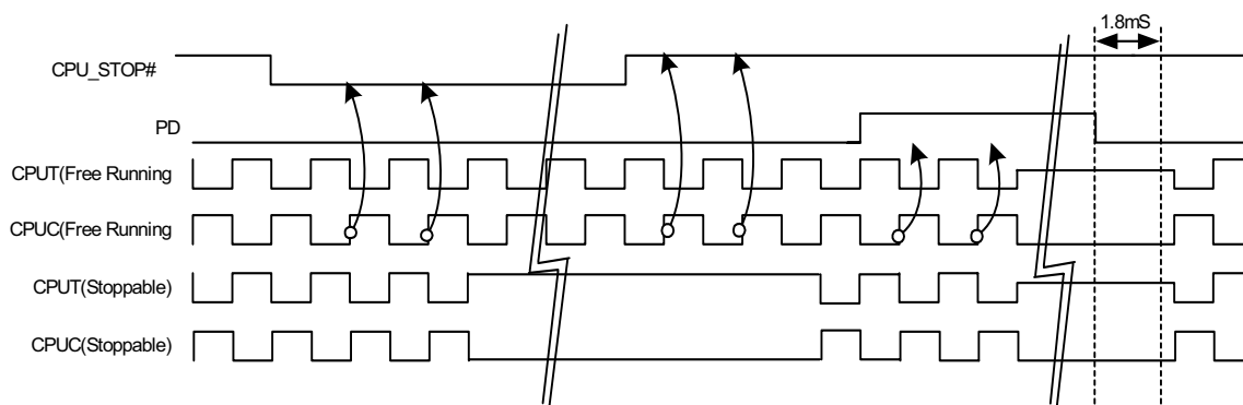
Figure 7. CPU_STOP# = Driven, CPU_PD = Driven
