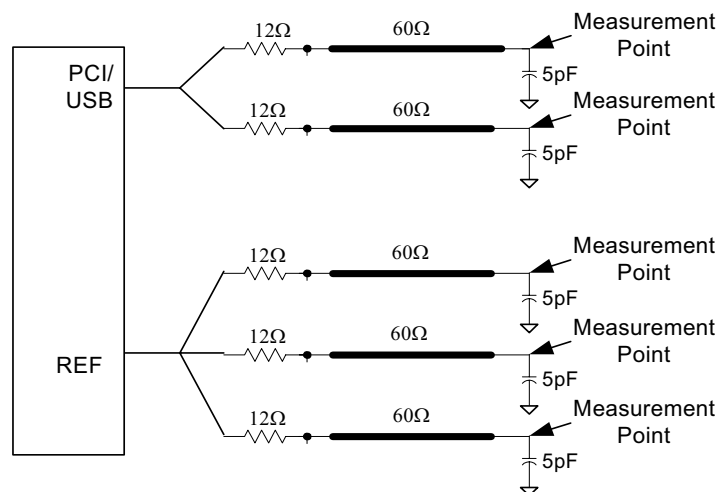
Figure 12. Single-ended Load Configuration
