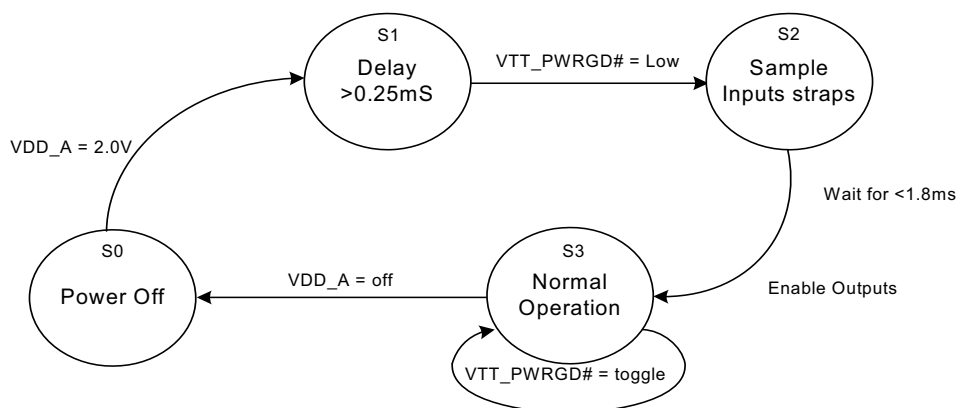
Figure 11. Clock Generator Power-up/Run State Diagram
