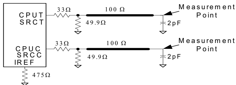
Figure 13. 0.7V Load Configuration
