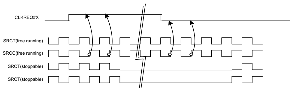
Figure 9. CLK_REQ#[0:1] Assertion/Deassertion Waveform
