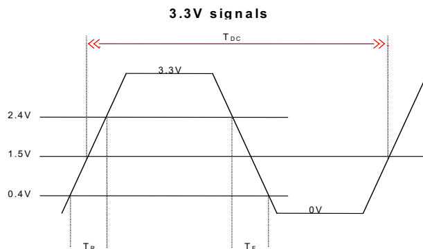
Figure 14. Single-ended Output Signals (for AC Parameters Measurement)
