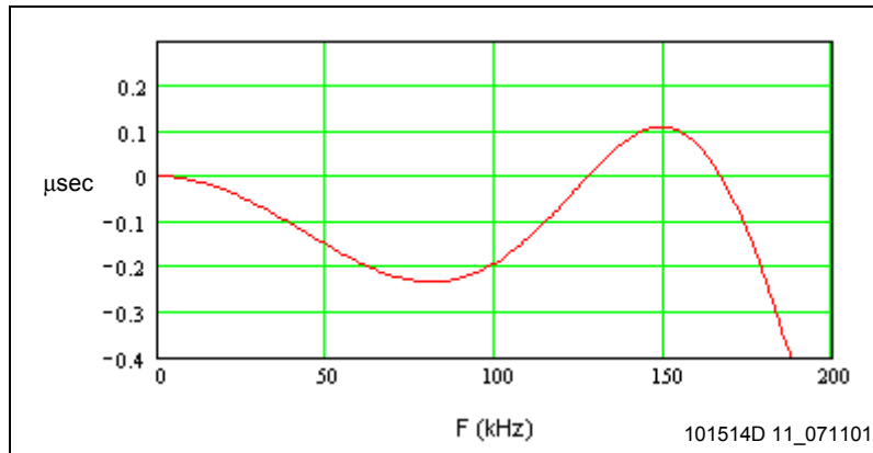
Figure 13. Typical Differential Delay Response
