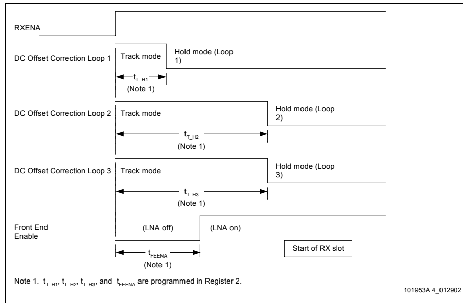
Figure 5. DC Offset Correction Timing (LNA On During Part of the DC Offset Correction Sequence)
