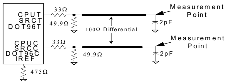
Figure 8. 0.7V Single-ended Load Configuration
