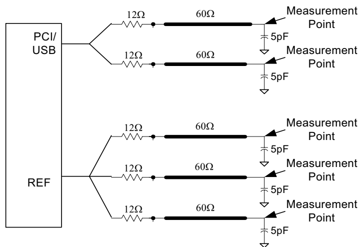
Figure 7. Single-ended Load Configuration
