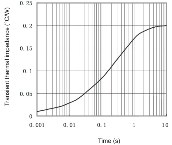
Fig.2 Thermal Impedance (junction to case)
