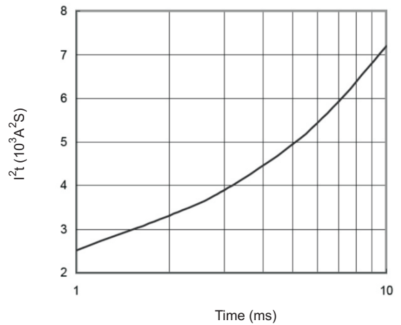
Fig.6 I^2t characteristic
