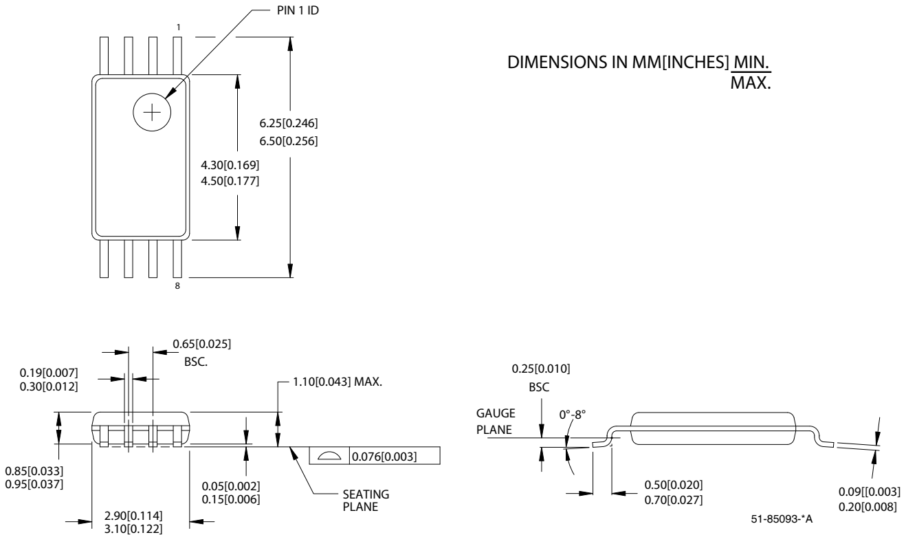
Figure 6. 8-Pb Thin Shrunk Small Outline Package (4.40 MM Body) Z8
