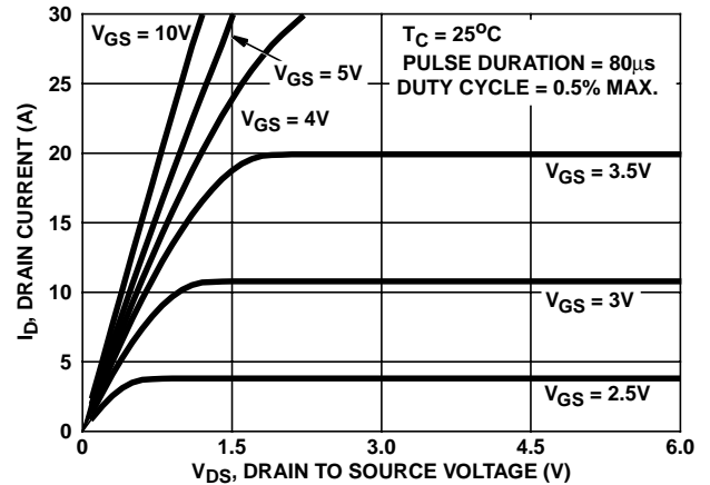
FIGURE 7. SATURATION CHARACTERISTICS
