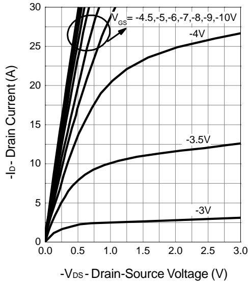
Output Characteristics
