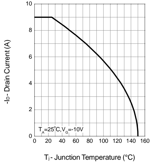
Drain Current
