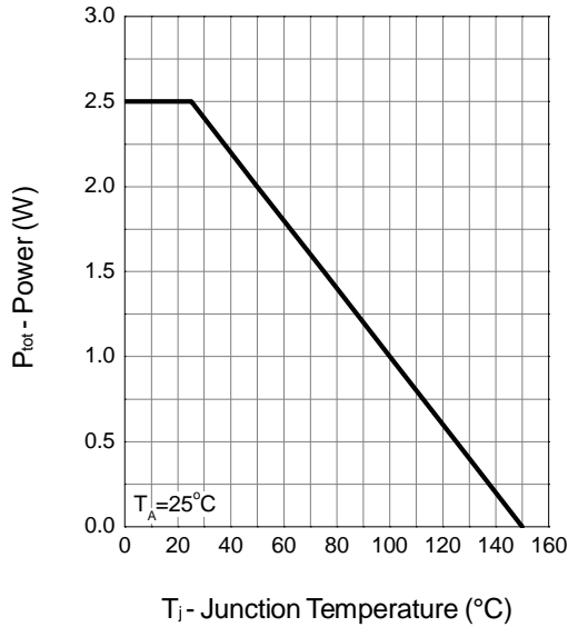
Power Dissipation
