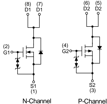
N-Channel
