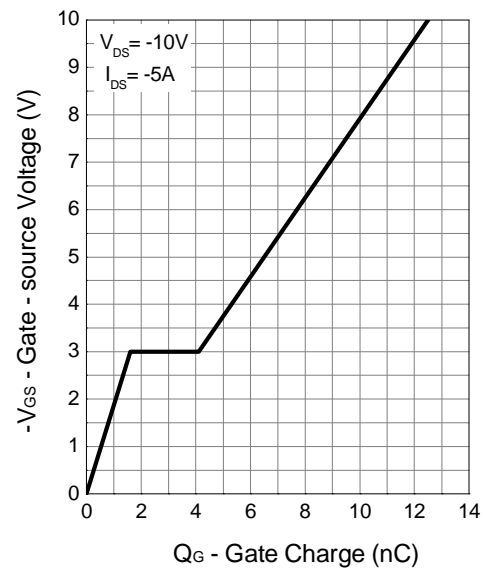
Gate Charge
