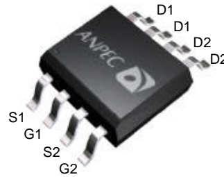
Top View of SOP – 8
