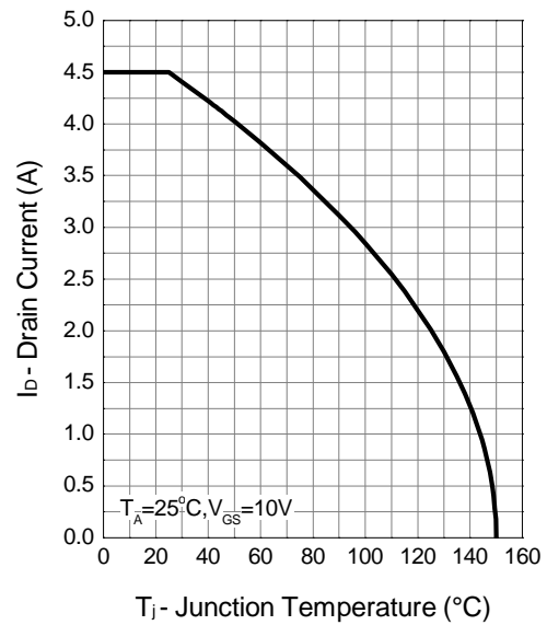
Drain Current
