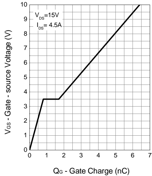
Gate Charge
