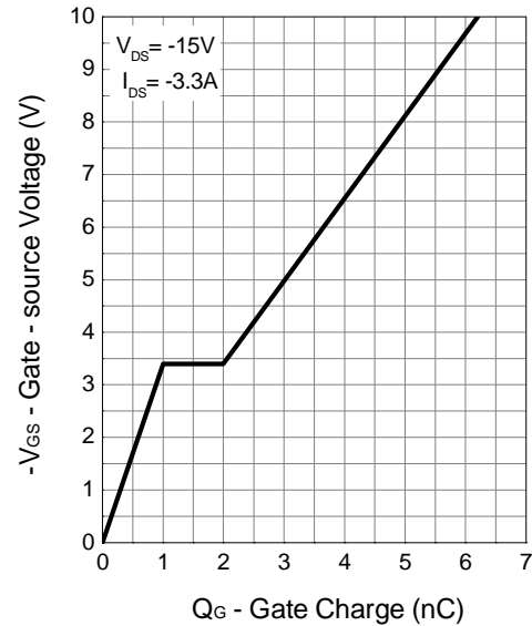
Gate Charge
