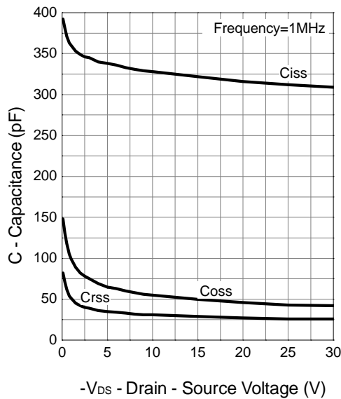
Capacitance
