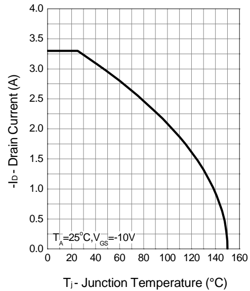
Drain Current
