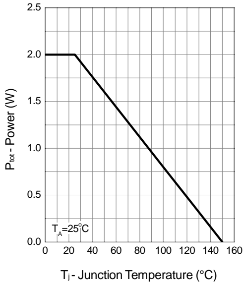
Power Dissipation
