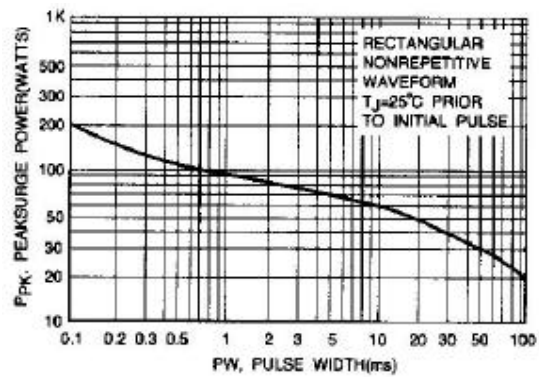
Fig. 6-MAXIMUM SURGE POWER
