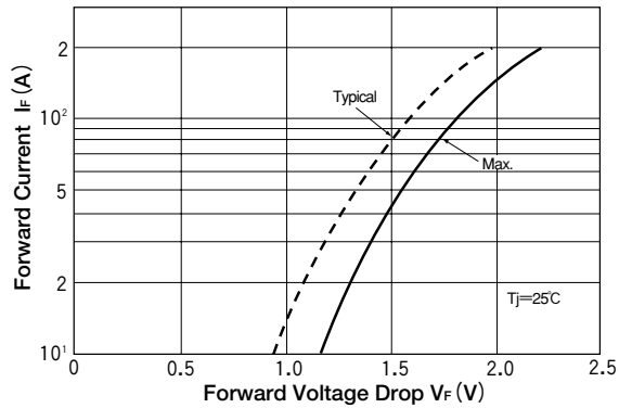
Forward Characteristics
