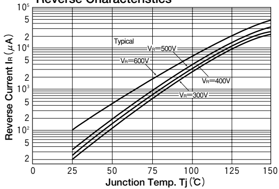
Reverse Characteristics
