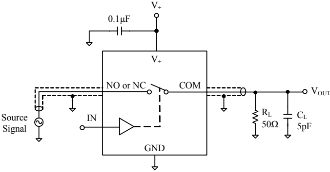
Test Circuit 7. Off Isolation
