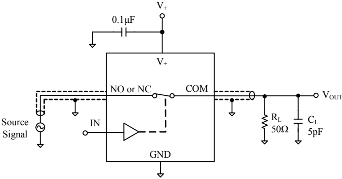
Test Circuit 8. Bandwidth
