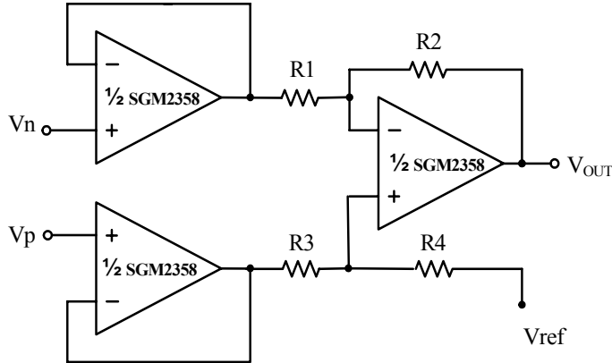
Figure 5. Instrumentation Amplifier
