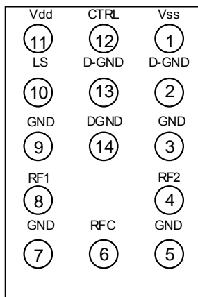
Figure 2. Die Top View (Bump Side Up)
