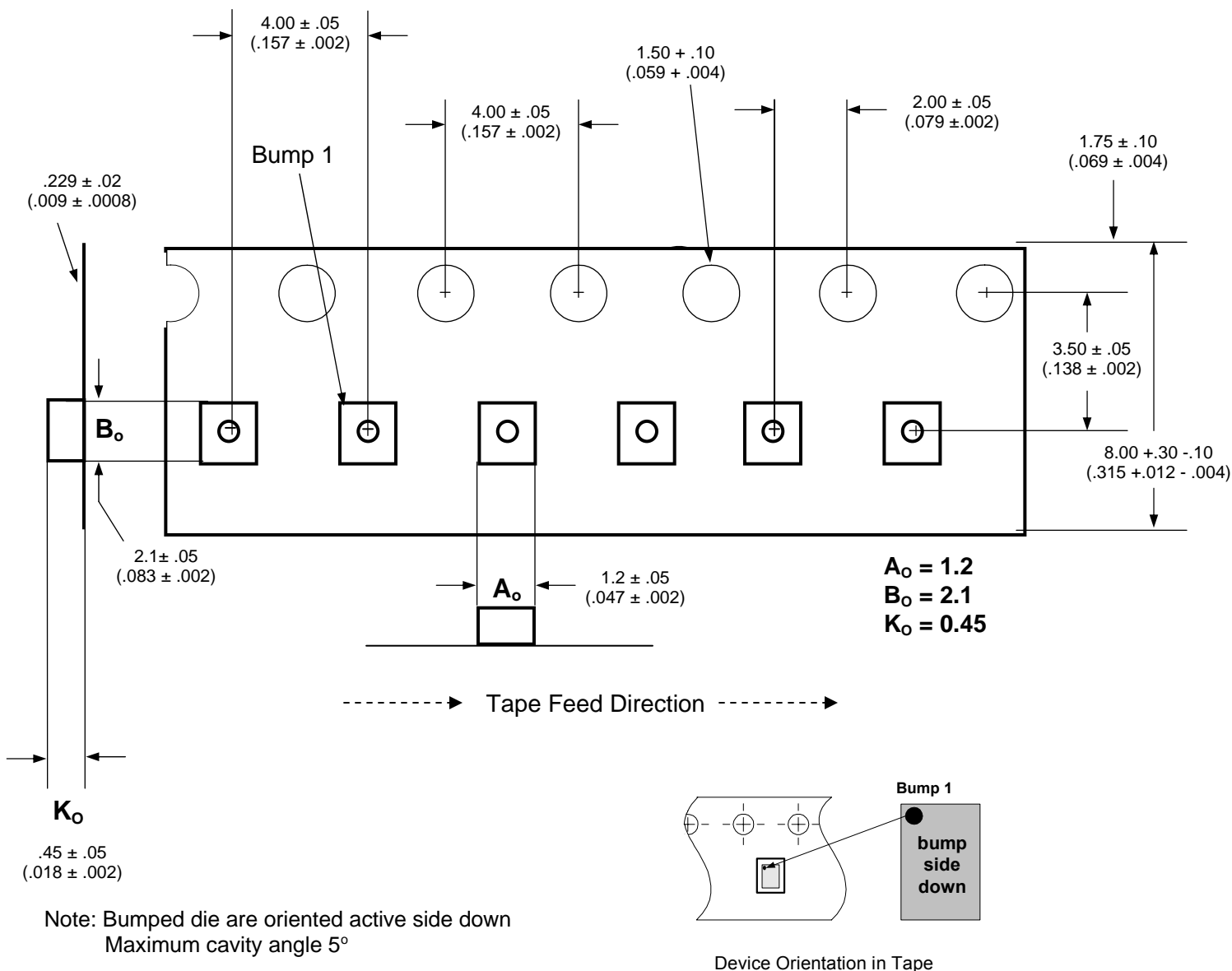
Figure 18. Tape and Reel Specifications
