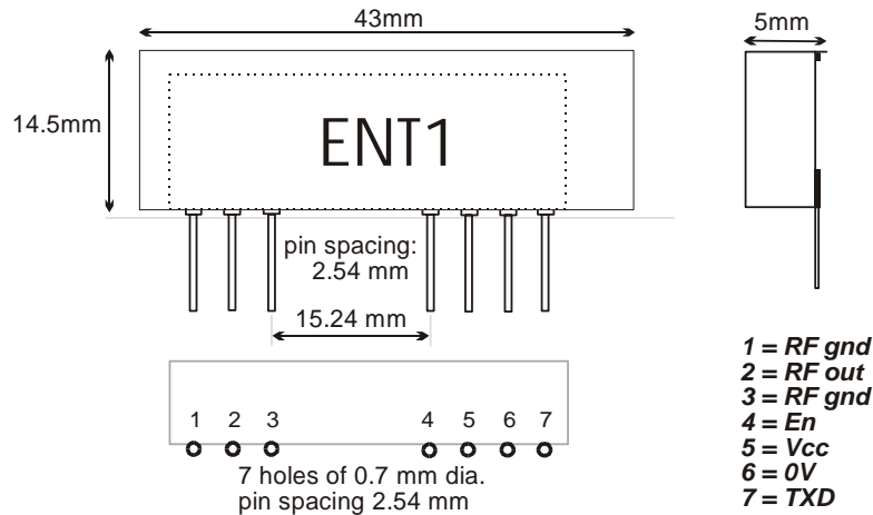
Figure 3: ENT1 pin-out and dimension
