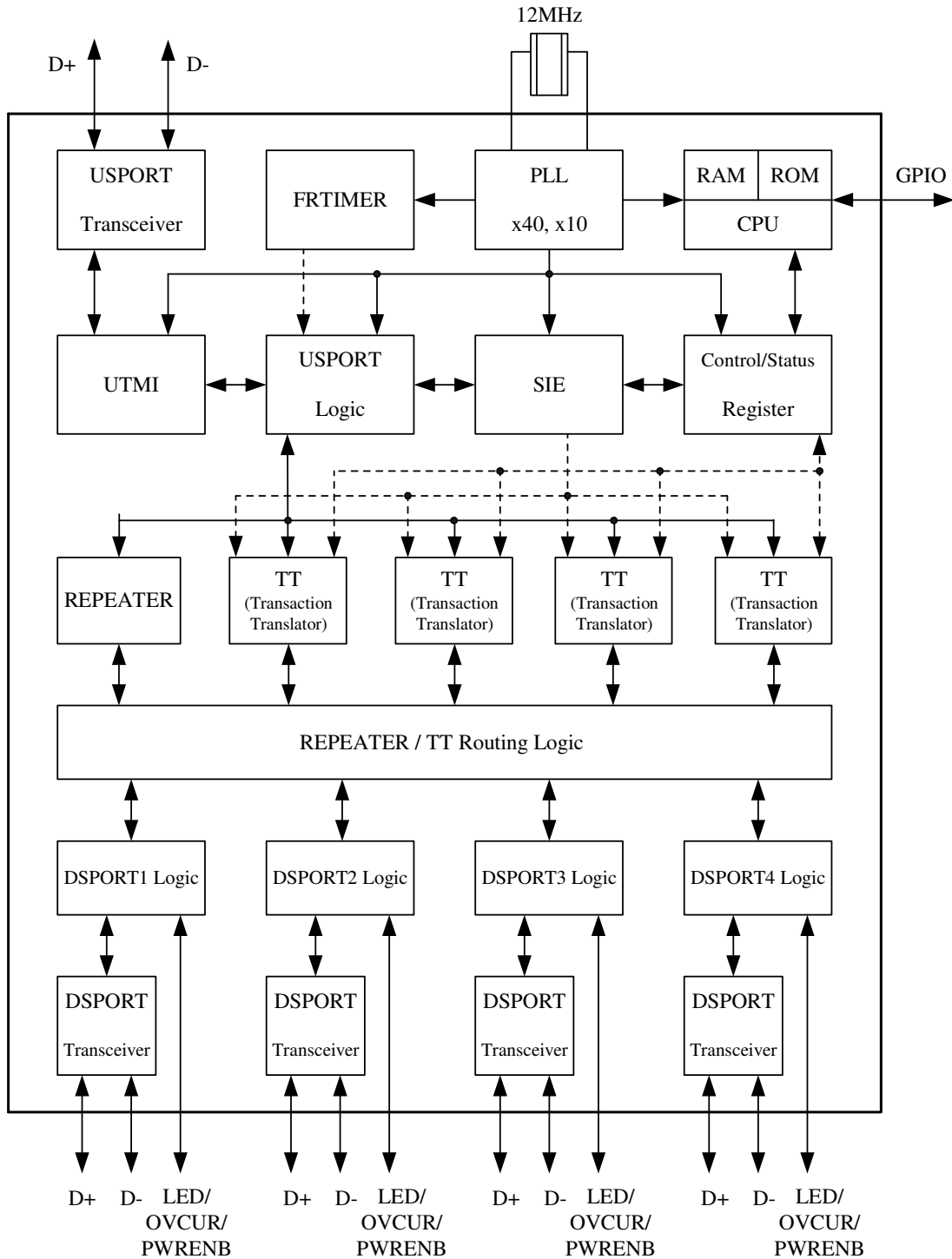
Figure 4.1 - GL852 Block Diagram (multiple TT)
