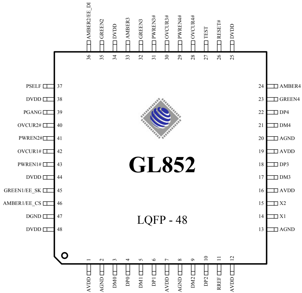
Figure 3.2 – GL852 48 Pin LQFP Pinout Diagram
