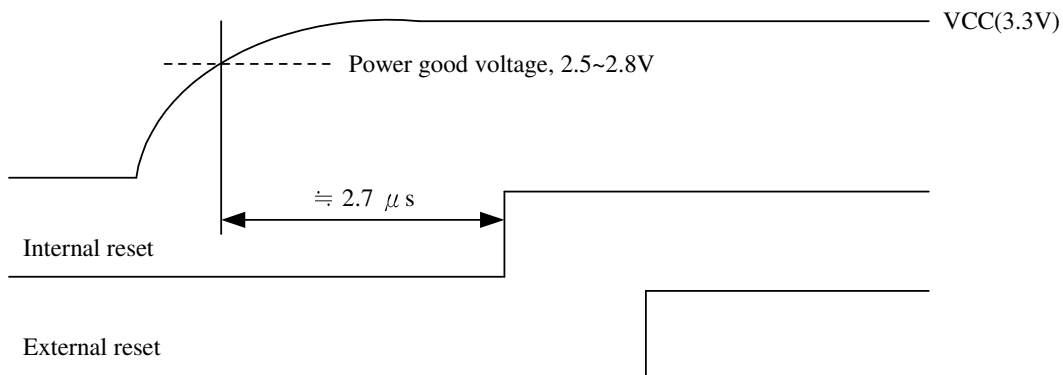
Figure 5.4 - Power on sequence of GL852
