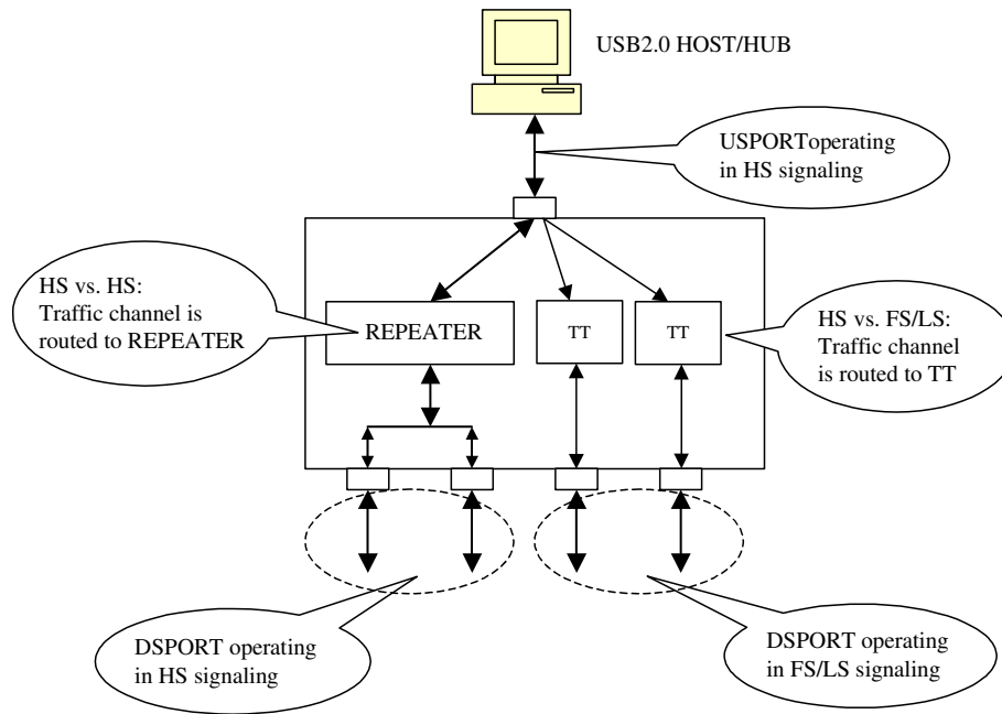
Figure 5.2 - Operating in USB 2.0 scheme
