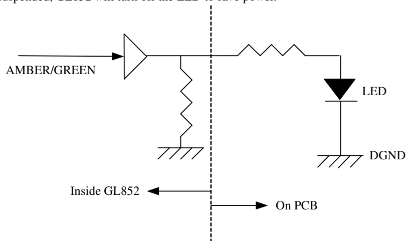
Figure 5.8 - LED Connection
