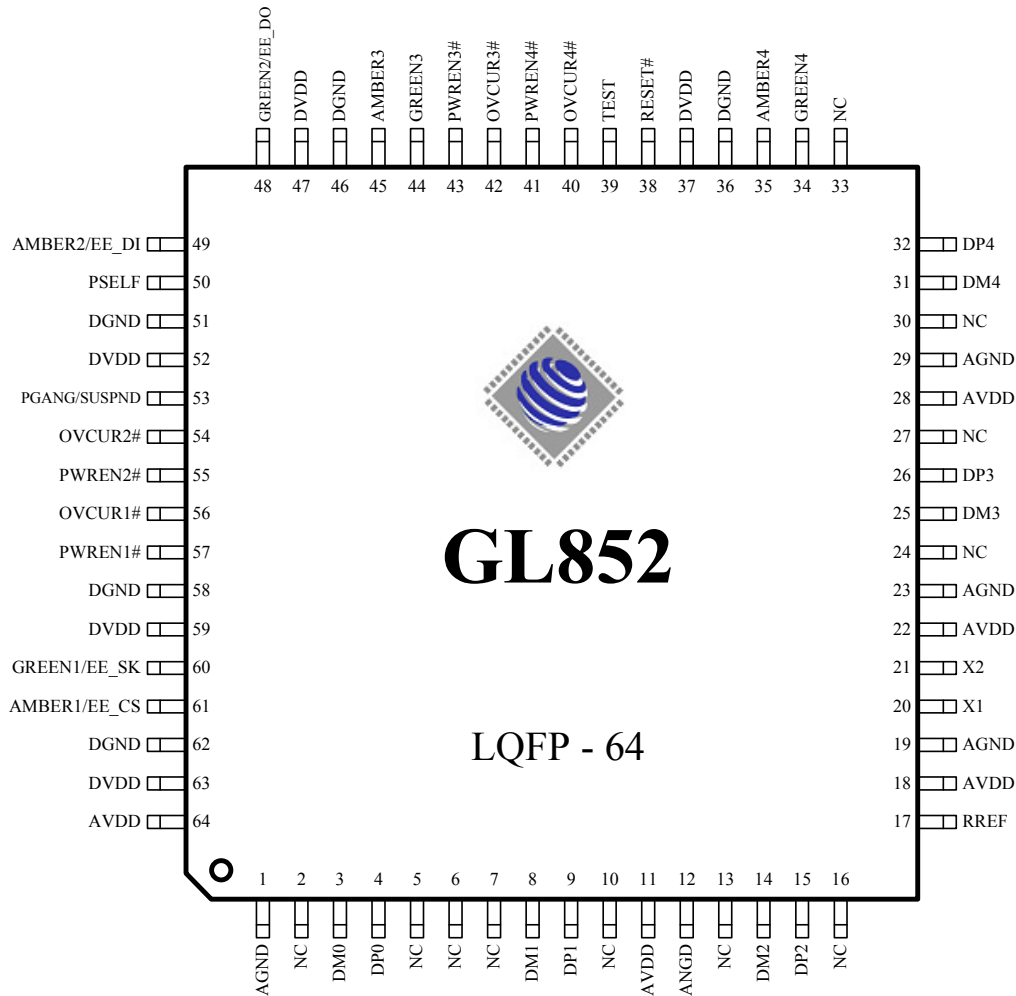
Figure 3.1 – GL852 64 Pin LQFP Pinout Diagram
