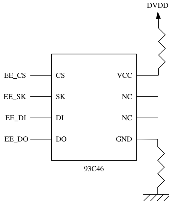
Figure 5.9 - Schematics Between GL852 and 93C46
