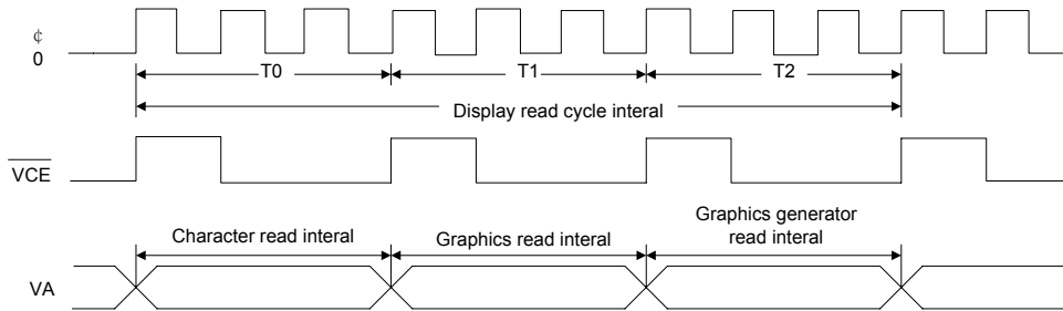
Figure 7-15: Display Memory Basic Read Cycle
