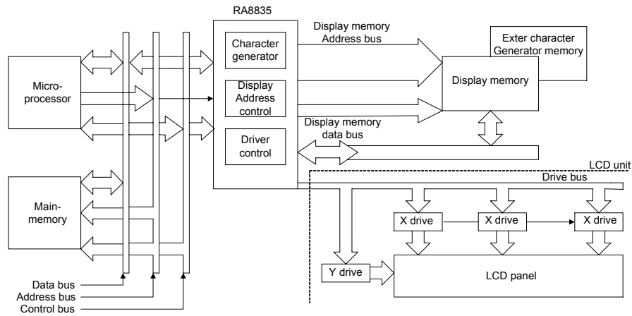
Figure 8-5: System Block Diagram
