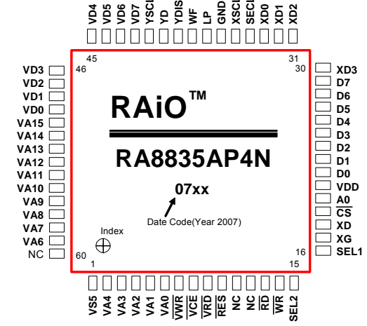
Figure 4-2: RA8835AP4N (TQFP-60 Pin)
