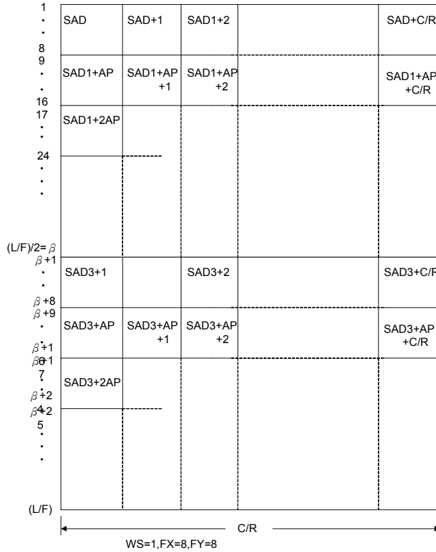
Figure 7-14: Two-panel Display Address Indexing
