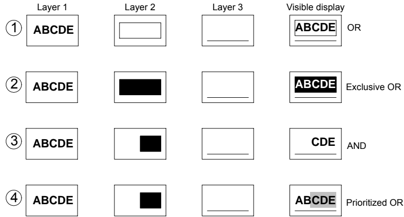
Figure 6-18: Combined Layer Display
