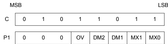
Figure 6-17: OVLAY Parameters
