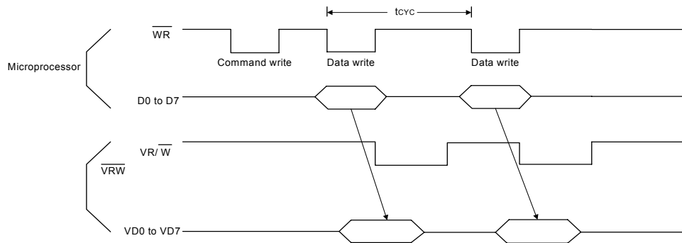
Figure 7-1A: Display Memory Write Cycle
