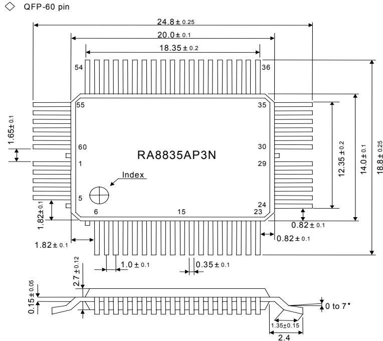
Figure 9-1: RA8835AP3N (Unit: mm)
