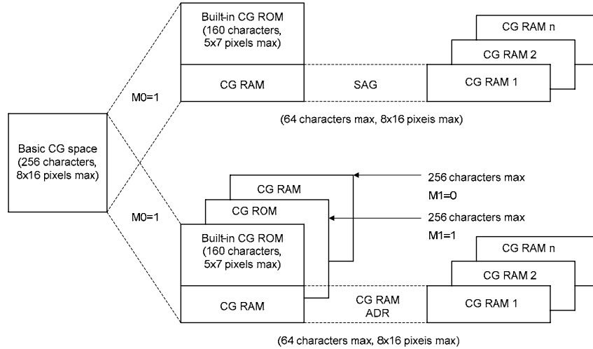
Figure 7-27: Internal and External Character Mapping
