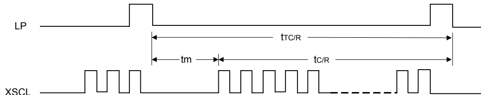
Figure 7-6: C/R to TC/R Time Difference
