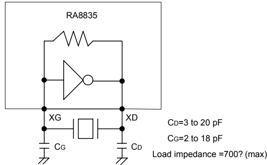
Figure 7-4: Crystal Oscillator
