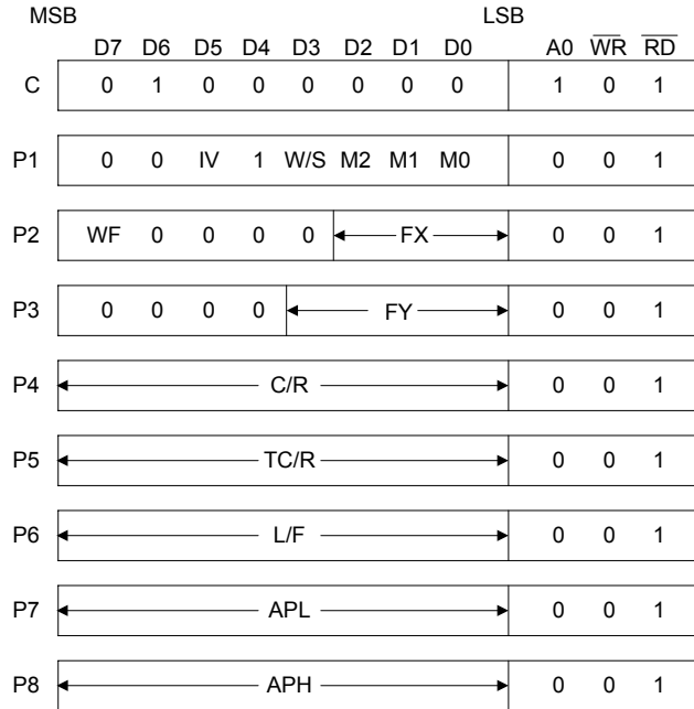
Figure 6-1: SYSTEM SET Instruction
