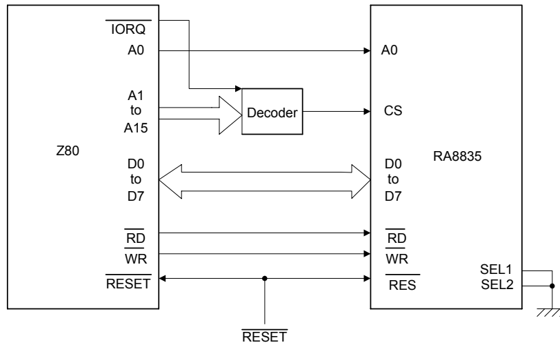
Figure 7-2A: Z80 to RA8835A Interface
