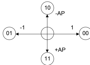
Figure 6-16: Cursor Direction
