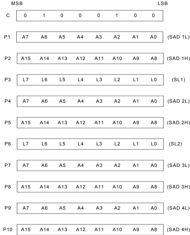
Figure 6-11: SCROLL Instruction Parameters
