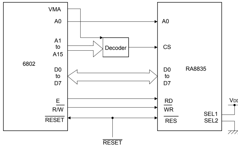
Figure 7-2B: 6802 to RA8835A Interface
