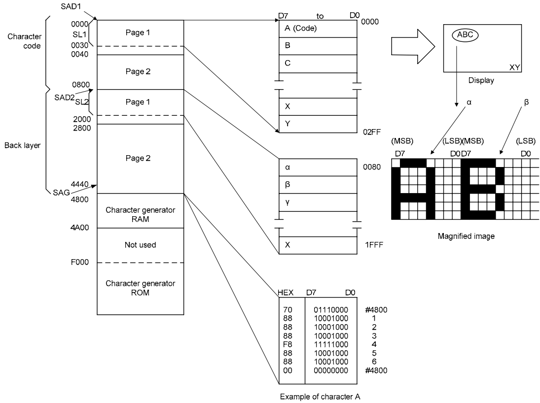
Figure 7-22: Memory Map and Magnified Characters
