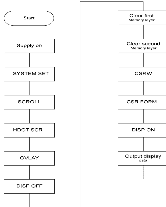
Figure 8-1: Initialization Procedure
