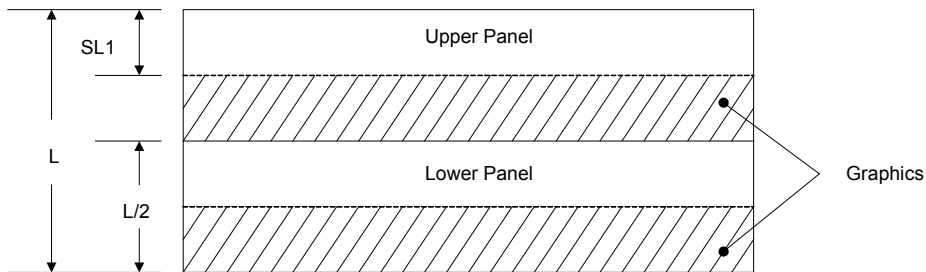
Figure 6-12: Two-panel Display Height
