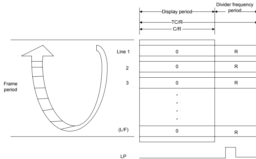
Figure 7-16: Relationship Between TC/R and C/R
