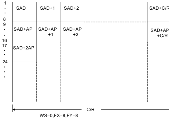
Figure 7-12: Character Position Parameters
