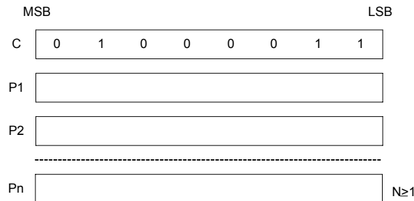
Figure 6-25: MREAD Parameters
