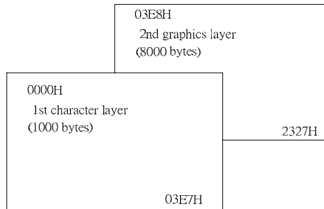
Figure 8-2: Character Over Graphics Layers
