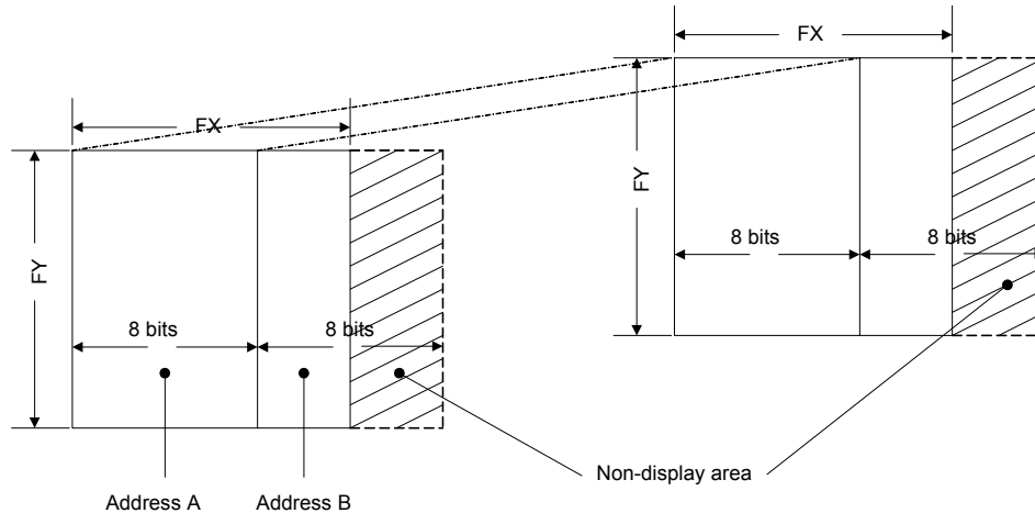
Figure 6-6: FX and FY Display Addresses
