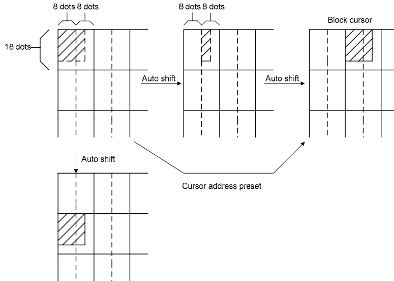
Figure 7-19: Cursor Movement
