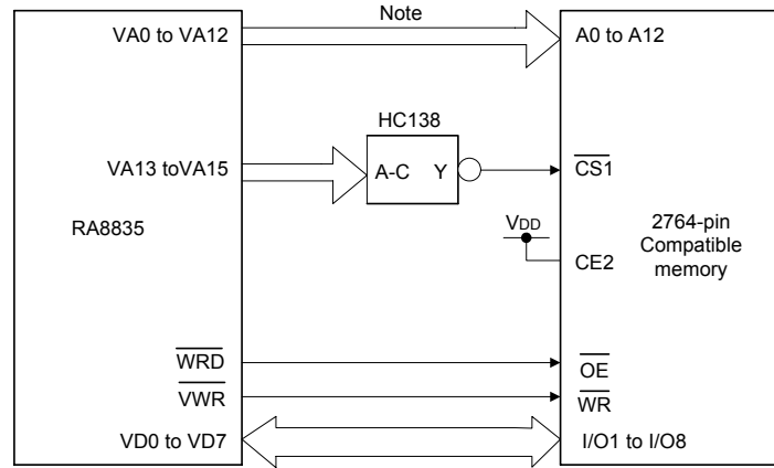
Figure 7-3: Static RAM Interface
