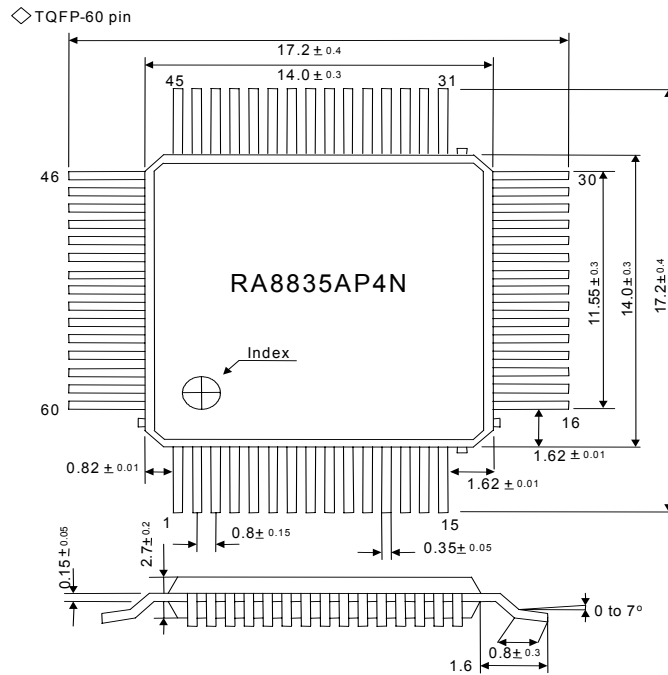
Figure 9-2: RA8835AP4N (Unit: mm)
