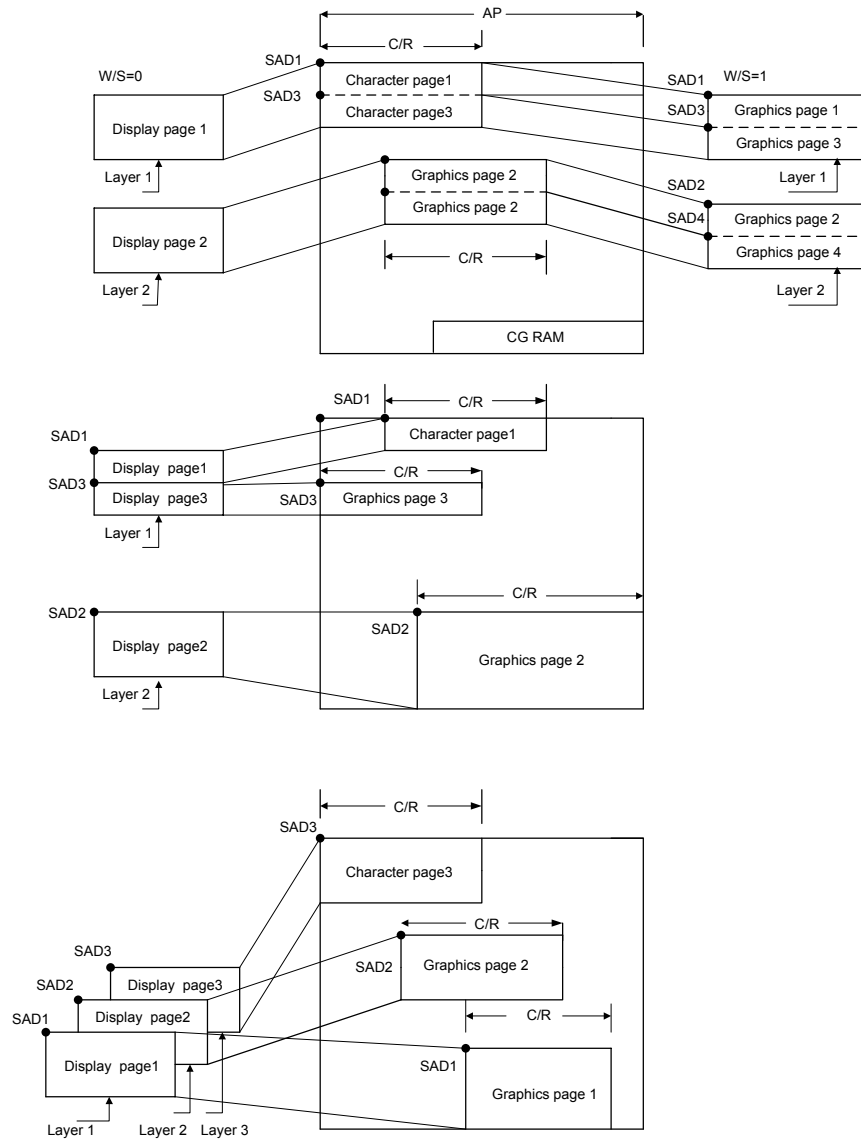
Figure 7-20: Display Layers and Memory
