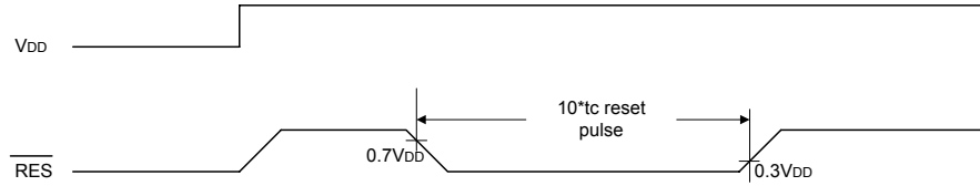
Figure 7-8: Reset Timing
