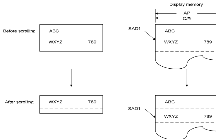
Figure 7-24: Inter-page Scrolling
