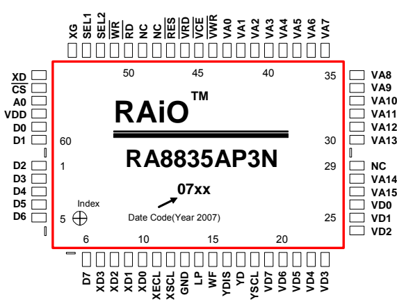
Figure 4-1: RA8835AP3N(QFP-60 Pin)
