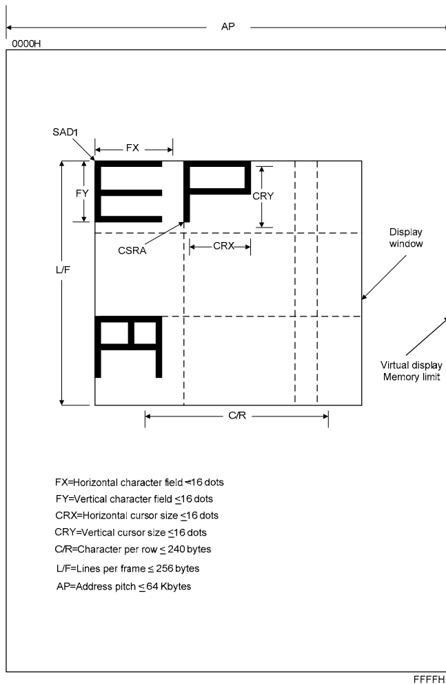
Figure 7-21: Display Windows and Memory
