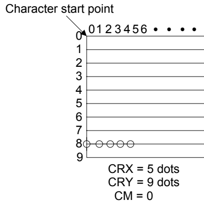
Figure 6-14: Cursor Size and Position
