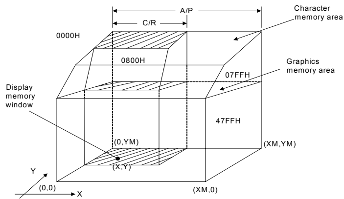
Figure 7-11: Virtual and Physical Screen Relationship
