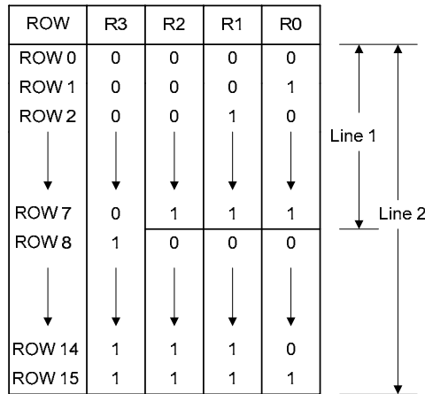
Figure 7-28: Row Select Address
