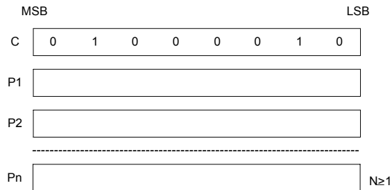
Figure 6-24: MWRITE Parameters
