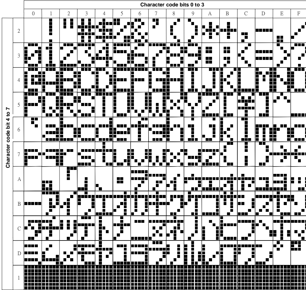
Figure 8-14: On-chip Character Set
