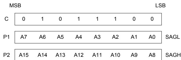
Figure 6-19: CGRAM ADR Parameters
