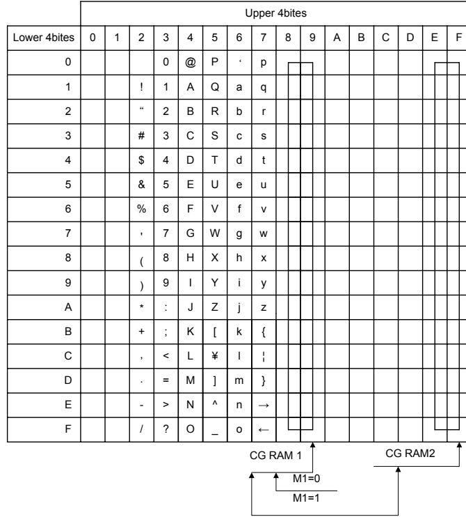
Figure 7-29: On-chip Character Codes
