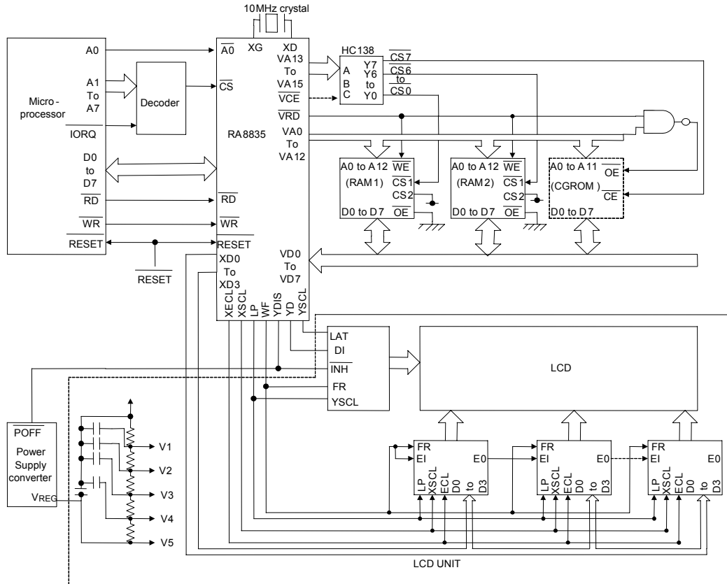
Figure 8-6: System Interconnection Diagram
