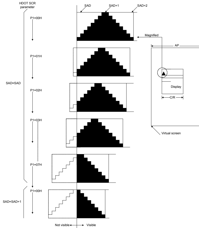
Figure: 8-7 HDOT SCR Example
