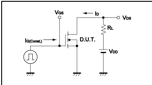
Fig.3-1 Avalanche Measurement Circuit
