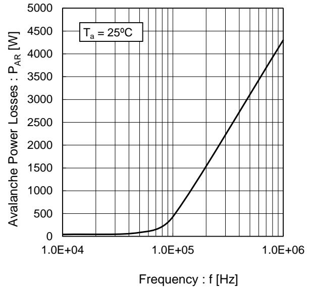
Fig.5 Avalanche Power Losses
