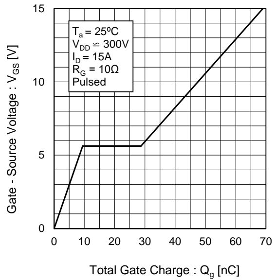
Fig.21 Dynamic Input Characteristics
