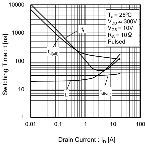
Fig.20 Switching Characteristics
