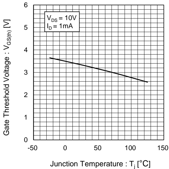
Fig.13 Gate Threshold Voltage vs. Junction Temperature
