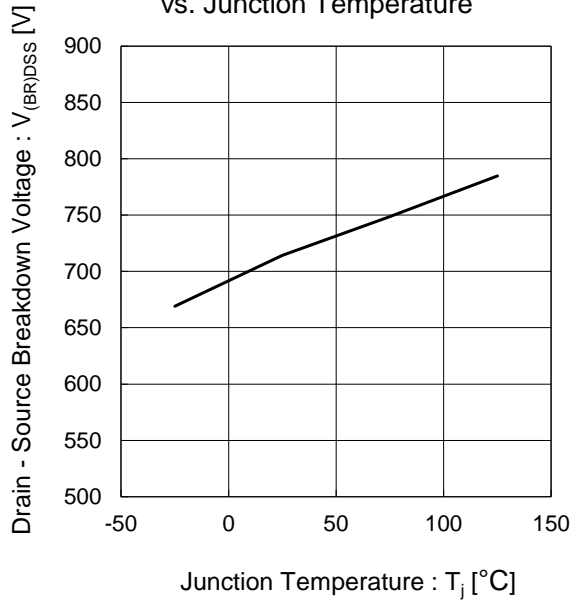
Fig.11 Breakdown Voltage vs. Junction Temperature
