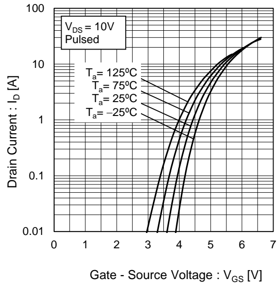
Fig.12 Typical Transfer Characteristics
