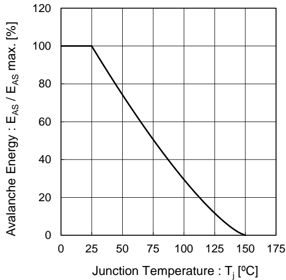
Fig.6 Avalanche Energy Derating Curve vs Junction Temperature
