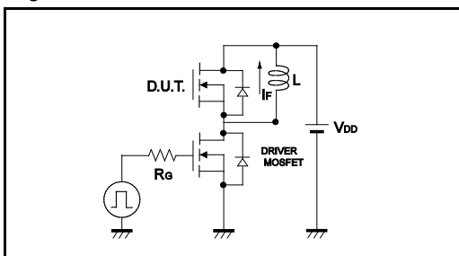
Fig.5-1 di/dt Measurement Circuit
