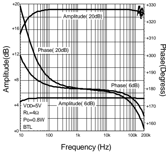
Frequency Response
