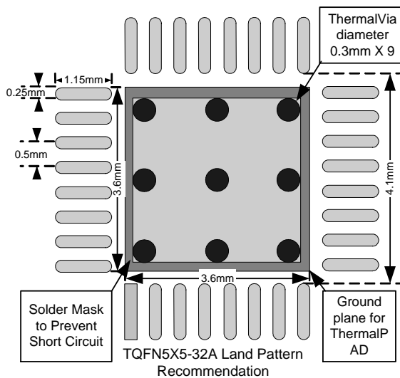
Figure 5. TQFN5x5-32A Land Pattern Recommendation
