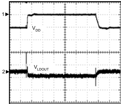
LDO Line Transient
