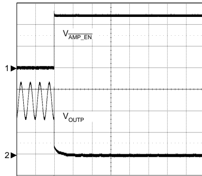
Speaker Disable
