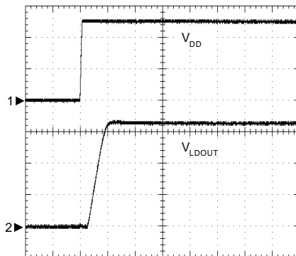
LDO Power On
