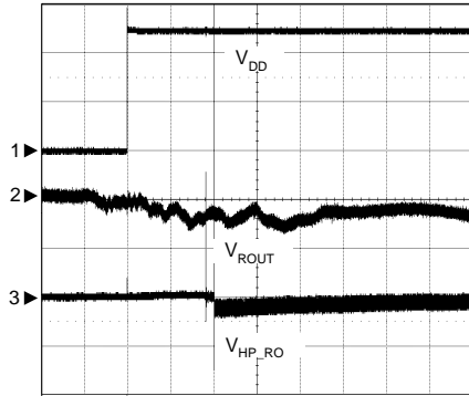
Power On
