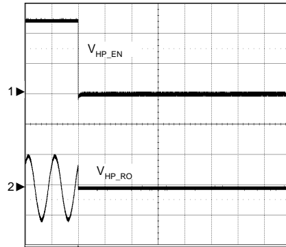
Headphone Disable
