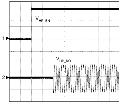
Headphone Enable
