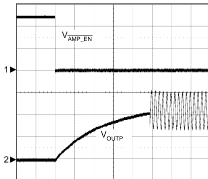
Speaker Enable
