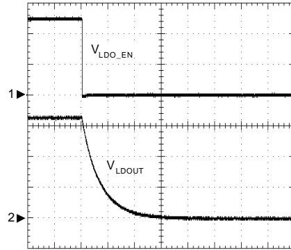
LDO Disable
