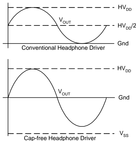
Figure 1: The Cap-Free Headphone Driver's Operation
