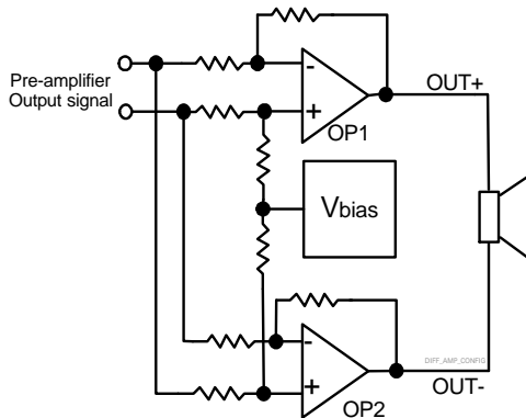
Figure 1: APA2057A internal configuration (each channel)
