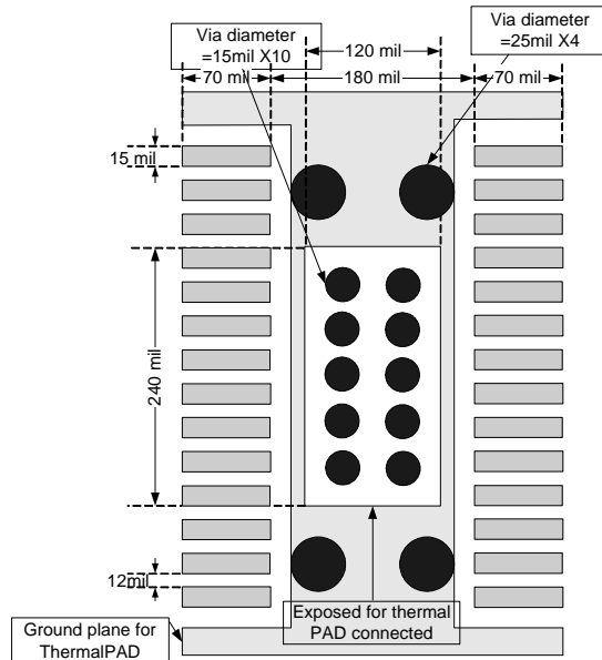
Figure 5: TSSOP-28P layout recommendation
