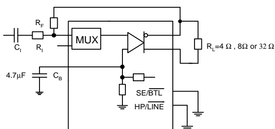
Figure 1. BTL Test Circuit
