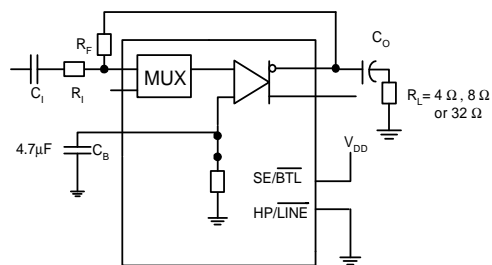
Figure 2. SE Test Circuit
