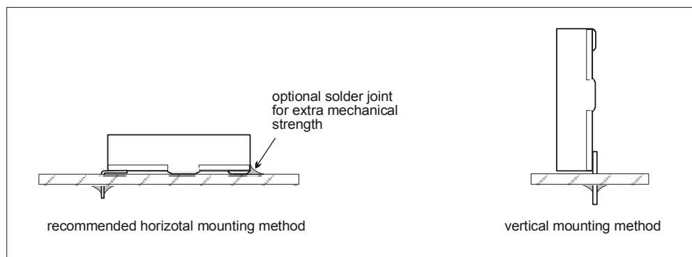
Figure 6: Module mounting options
