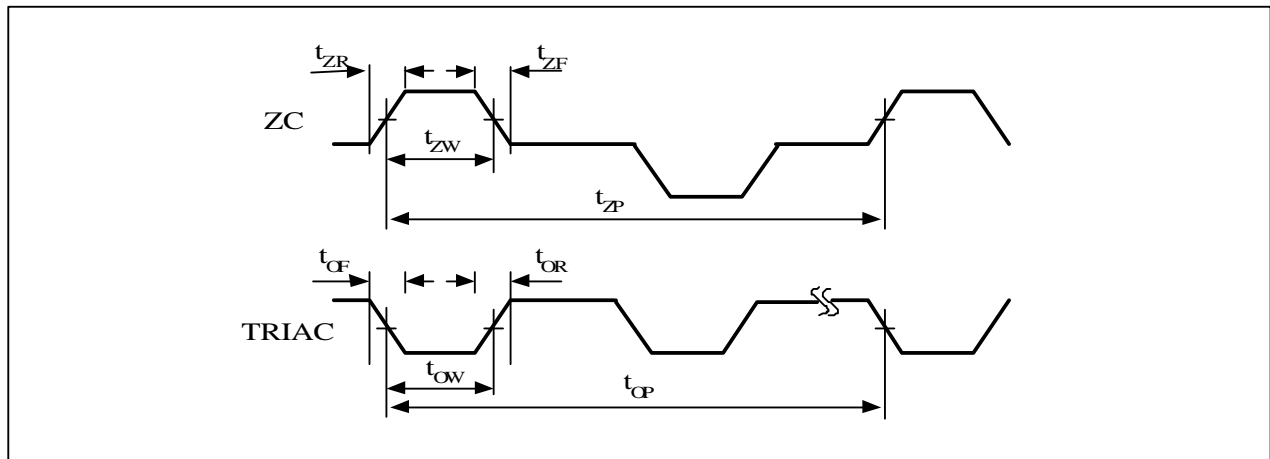
Figure 8. Timing Diagram
