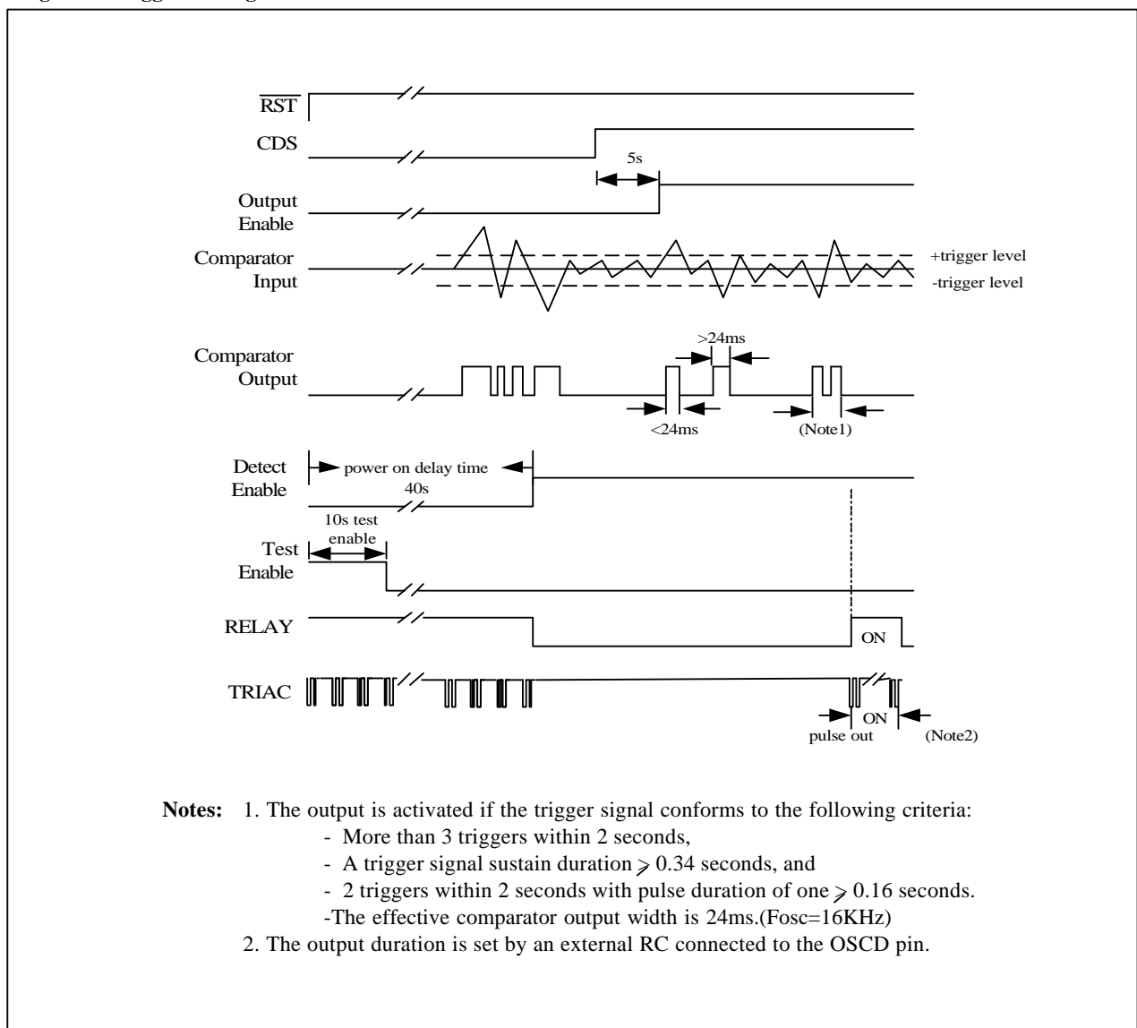
Figure 7. Trigger Timing
