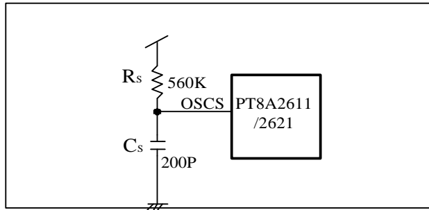
Figure 1. System Oscillator
