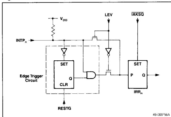
Figure 17. INTP Input
