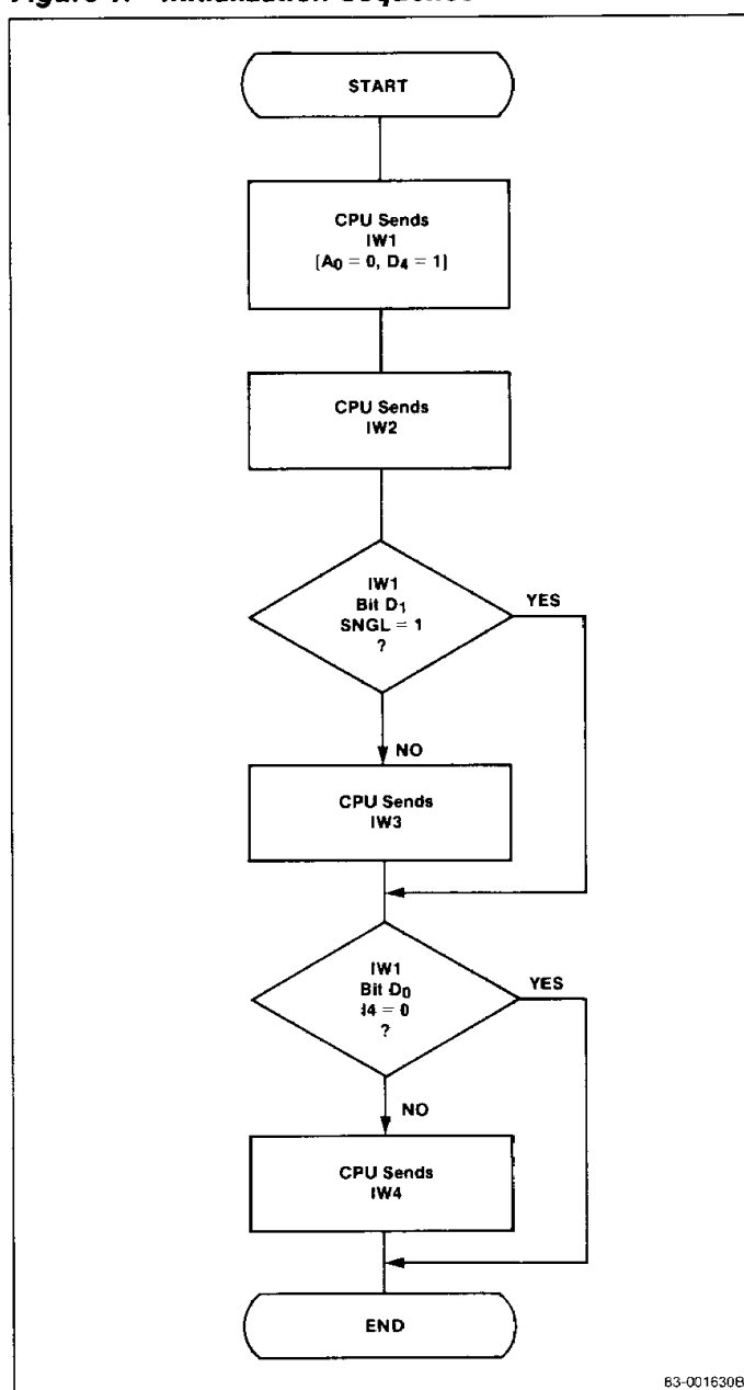
Figure 1. Initialization Sequence
