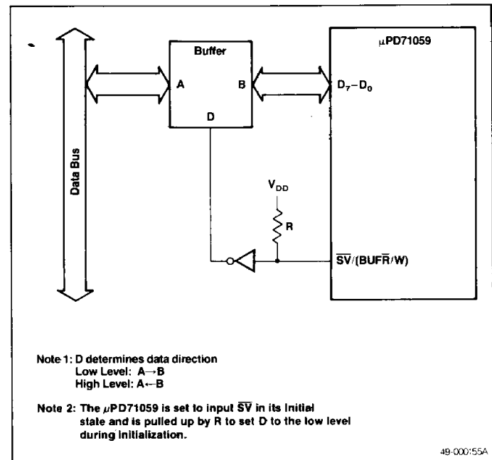
Figure 14. Buffer Mode
