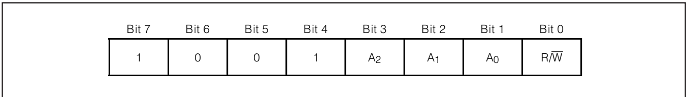
Figure 7. Address Byte
