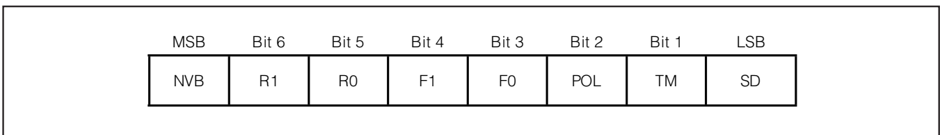
Figure 5. Configuration Register
