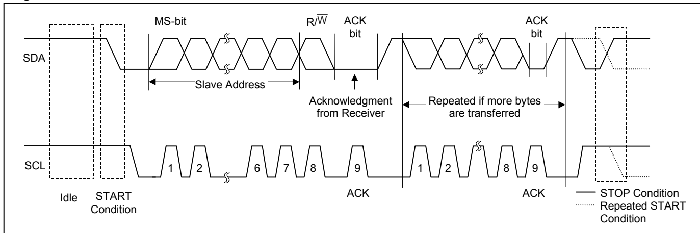
Figure 7. I 2 C Protocol Overview
