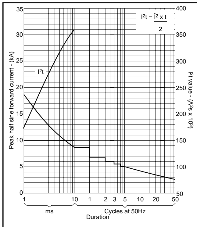
Fig.5 Surge (non-repetitive) forward current vs time (with 50% V_{RRM} at T_{case} 125^\circ\text{C} )
