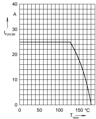
Fig. 5 Max. forward current at case temperature 180° sine
