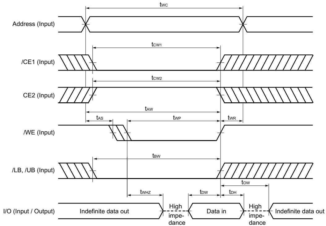
Write Cycle Timing Chart 1 (/WE Controlled)
