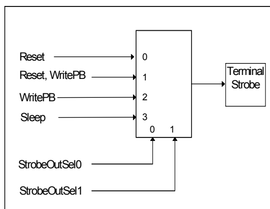
Figure 33 . Strobe Output
