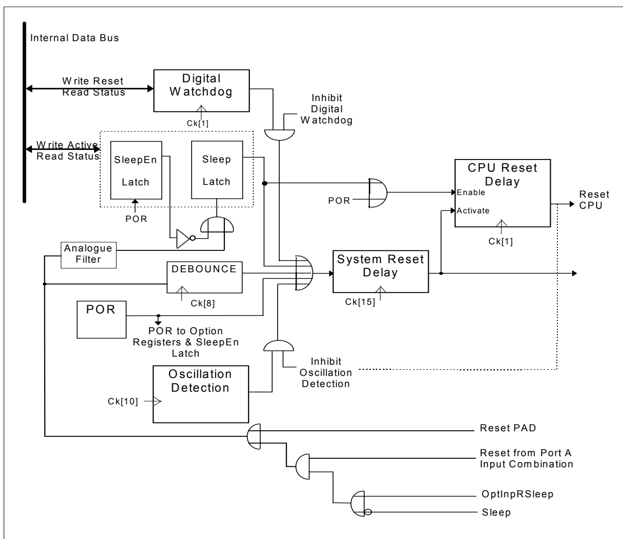
Figure 6. Reset Structure
