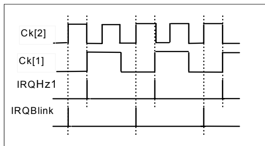
Figure 9. Prescaler Interrupts
