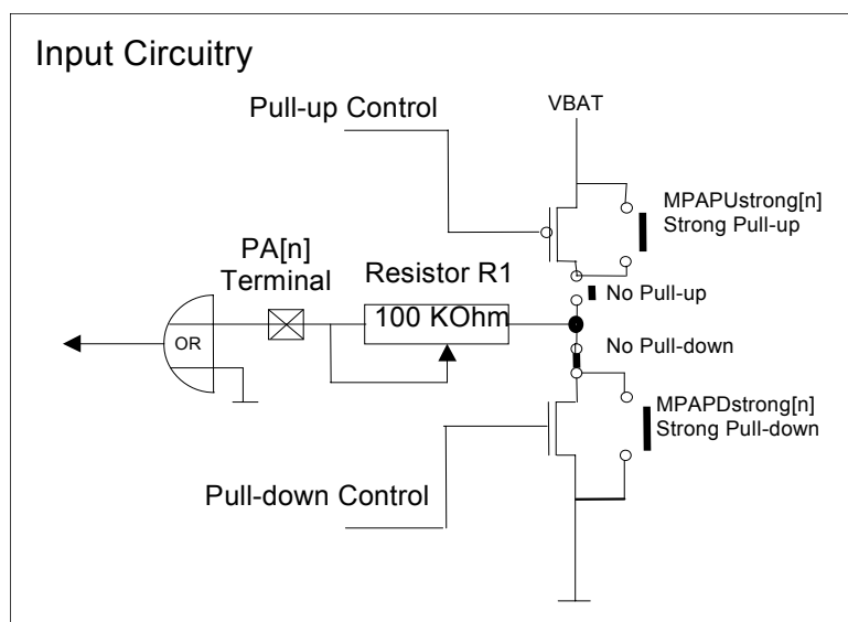
Figure 38. Port A Pull Options
