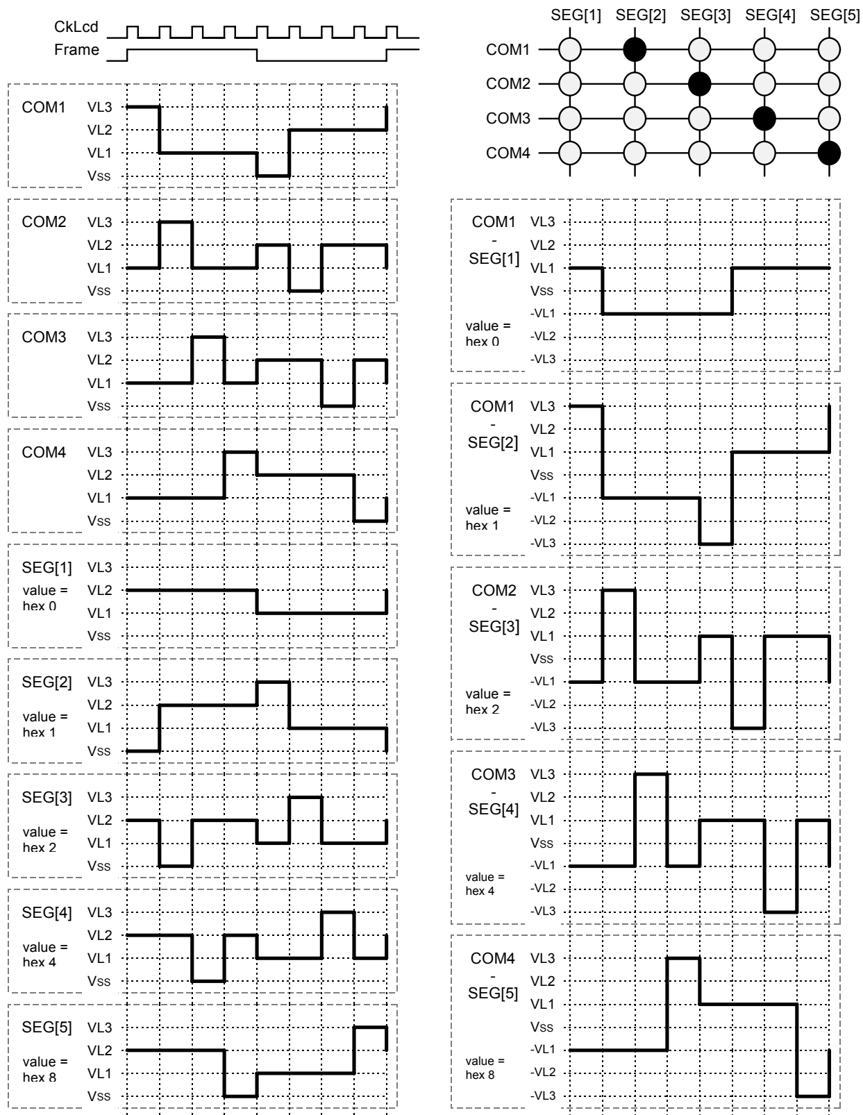
Figure 37 LCD Multiplexing Waveform
