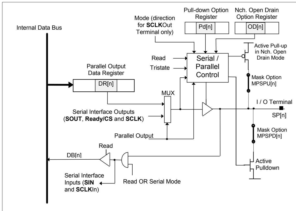
Figure 14. Port SP Terminal Configuration
