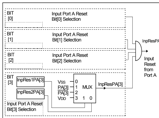
Figure 7. Input Port A Reset Structure
