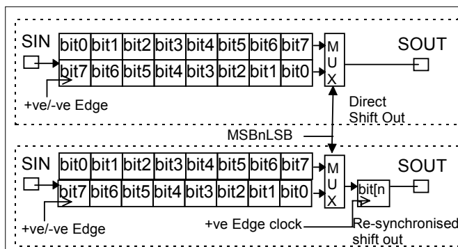
Figure 16. Direct or Re-Synchronized Output
