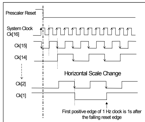
Figure 8. Prescaler Frequency Timing
