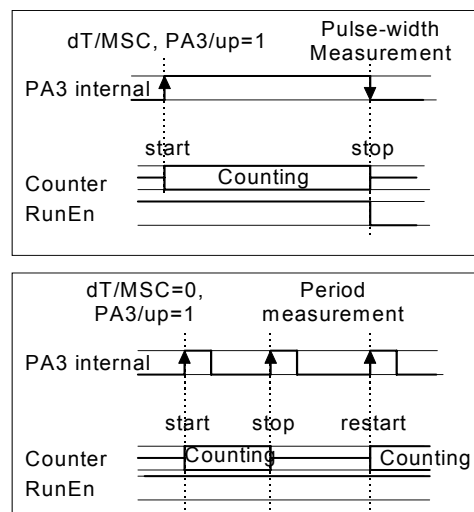
Figure 30. dT/MSC behavior
