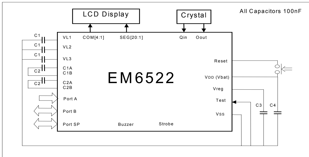
Figure 3. Typical Configuration
