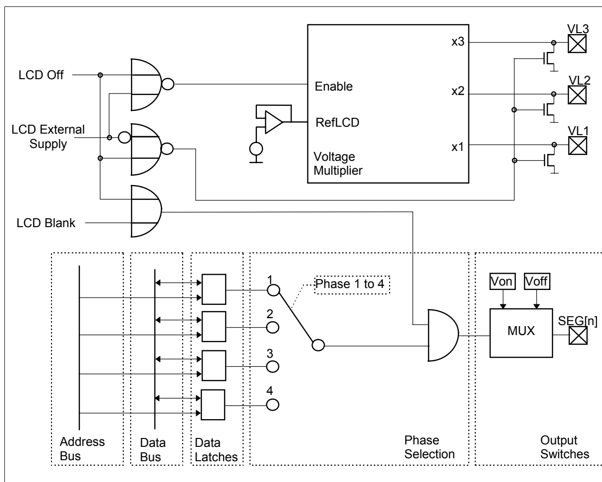
Figure 35. LCD Architecture
