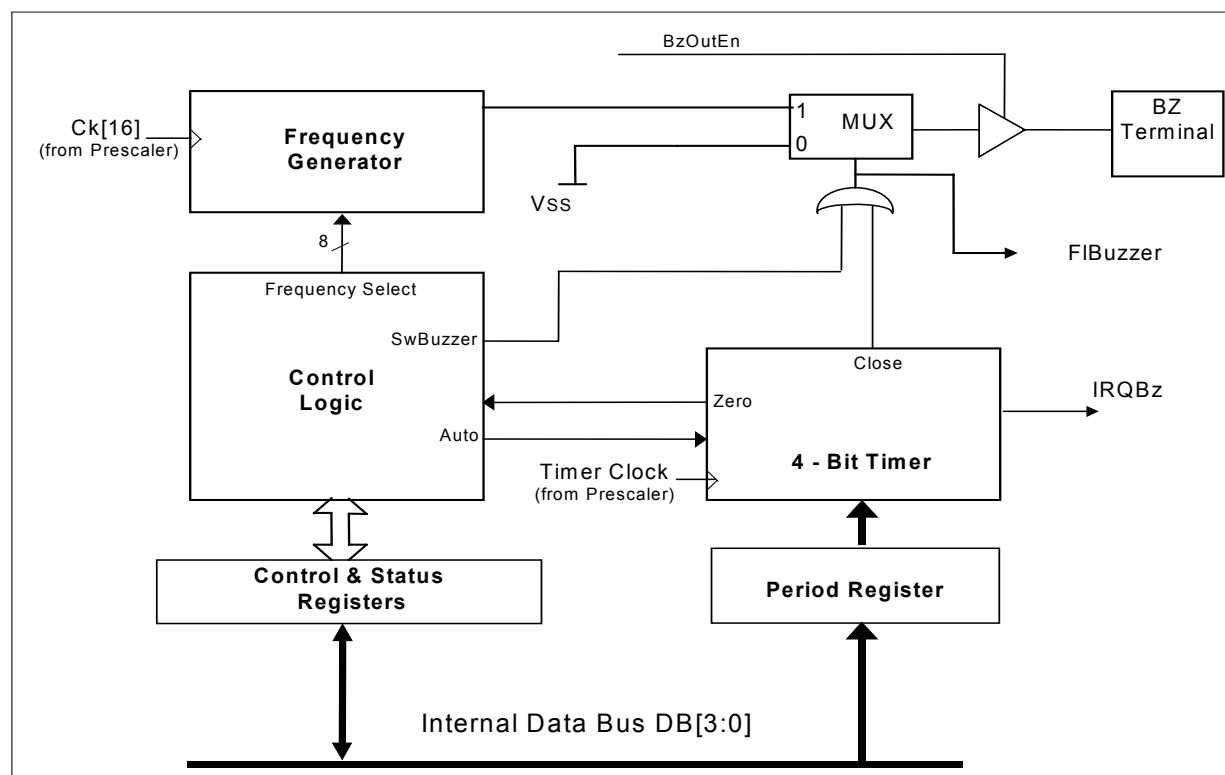
Figure 19. Melody Generator Block Diagram
