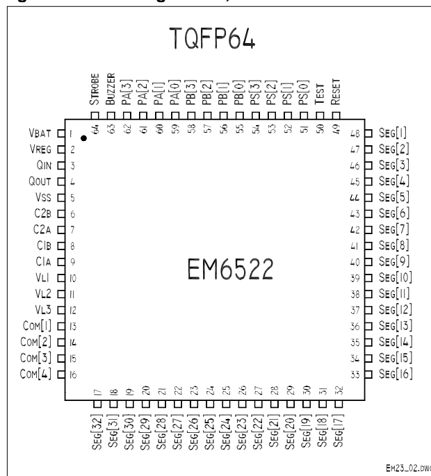
Figure 2. Pin Configuration, TQFP64 10 x 10 x 1 mm
