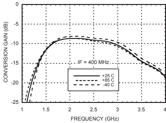
Conversion Gain vs. Temperature @ LO = +10 dBm
