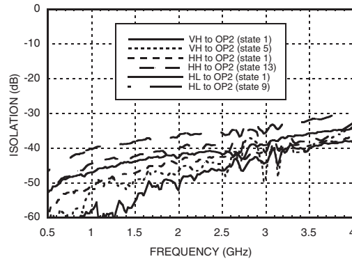
Isolation When VL is Connected to OP2*
