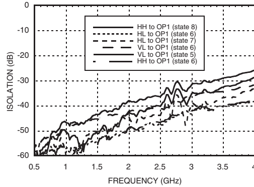
Isolation When VH is Connected to OP1*
