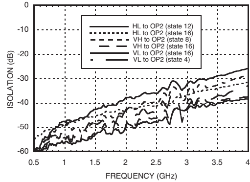
Isolation When HH is Connected to OP2*
