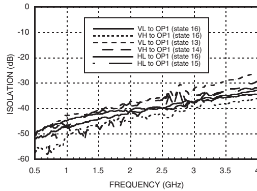
Isolation When HH is Connected to OP1*
