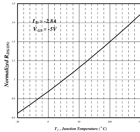
Fig 4. Normalized On-Resistance
