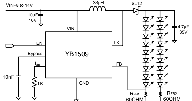
Figure 6. 2 Legs of 9 LEDs in a Series
