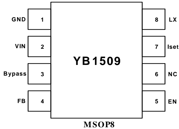
Figure 2. Pin configuration
