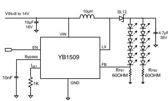
Figure 5. 2 Legs of 6 LEDs in a Series
