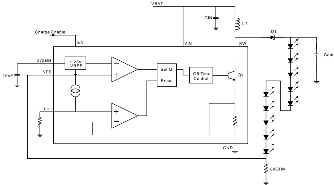
Figure 9. Block Diagram
