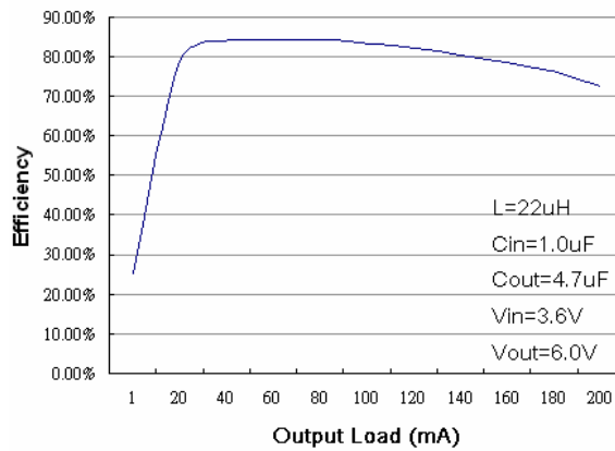
Efficiency vs Output Load (2)
