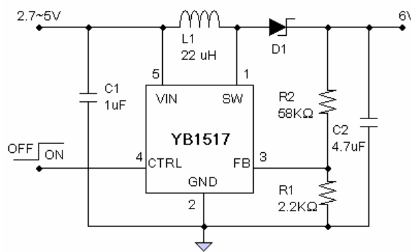
Figure 5: Typical Application Circuit
