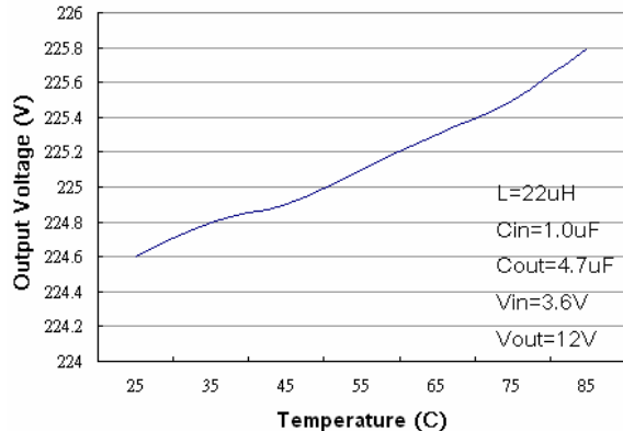
VFB Voltage vs Temperature
