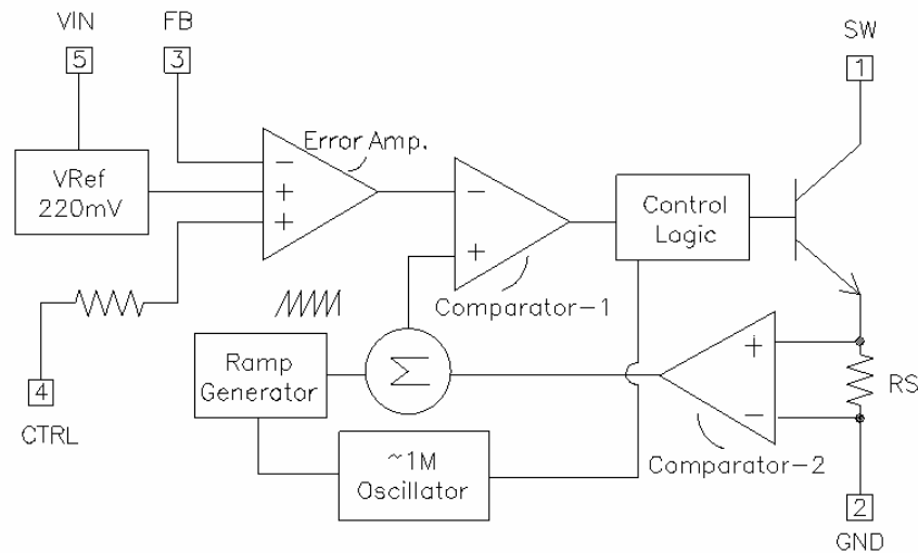
Figure 4: YB1517 Block Diagram
