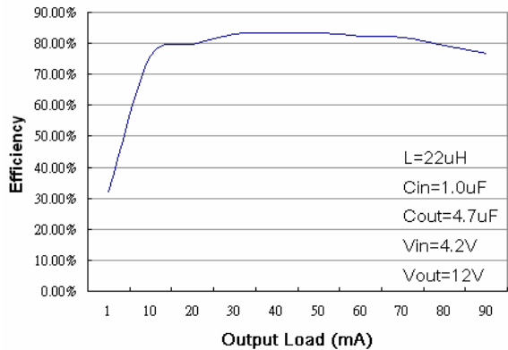
Efficiency vs Output Load (2)
