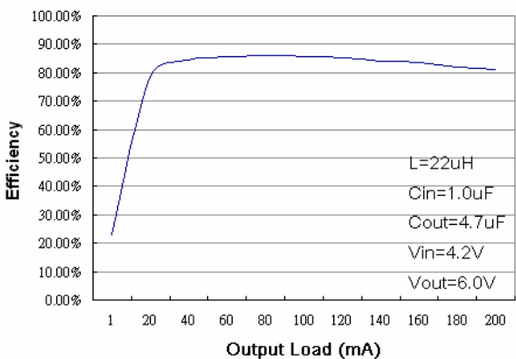
Efficiency vs Output Load (3)
