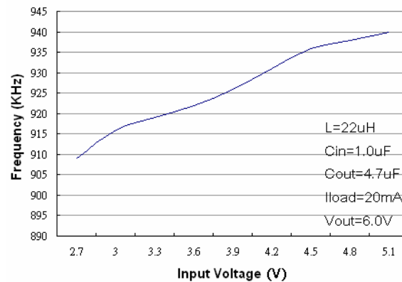
Frequency vs Input Voltage
