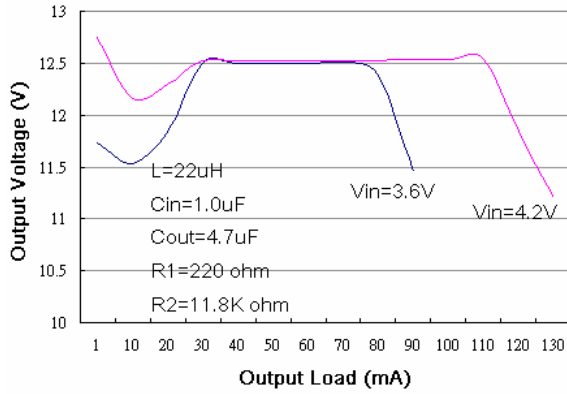
Output Voltage vs Output Load
