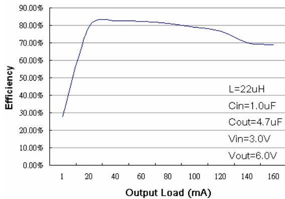
Efficiency vs Output Load (1)
