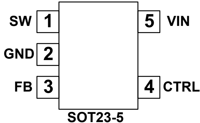
Figure 3: Pin Configuration
