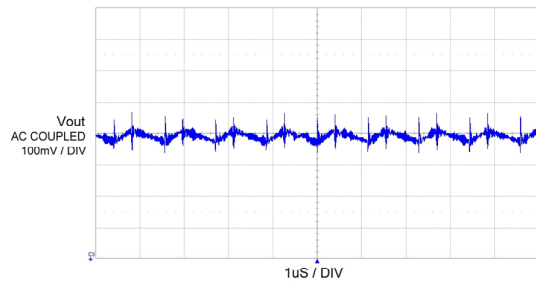
Output Ripple
