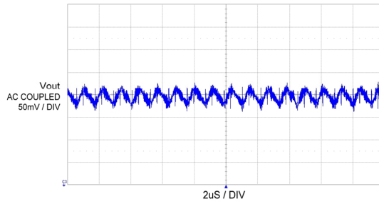
Output Ripple
