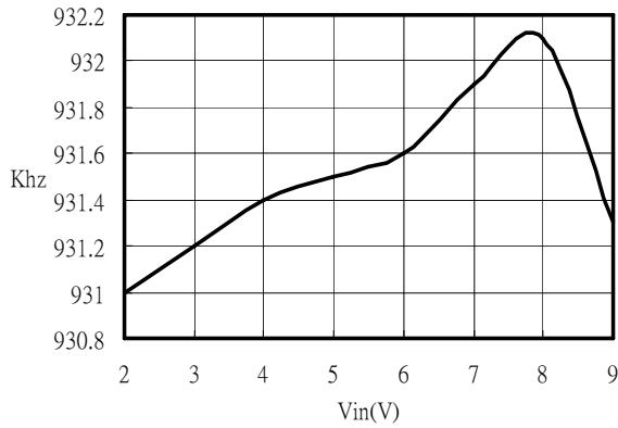
Switching Frequency
