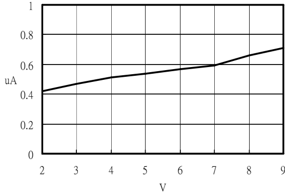
Supply Current (Vctrl = 0V)
