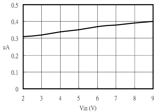
Switch Leakage Current
