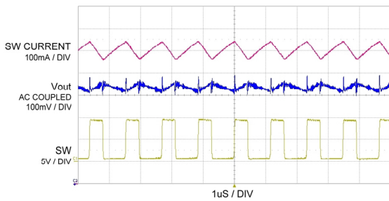
Output Waveform
