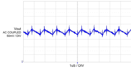
Output Ripple
