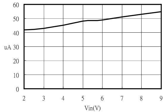
CTRL Pin Bias Current
