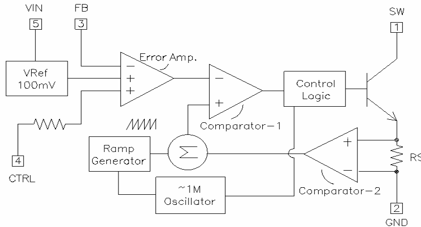
Figure 3: YB1522 Block Diagram
