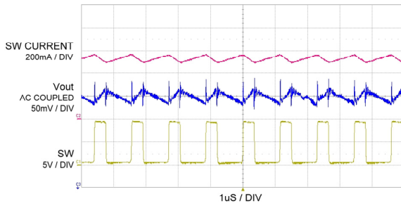
Output Waveform
