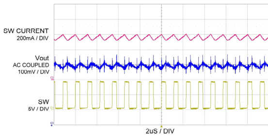
Output Waveform
