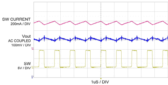
Output Waveform
