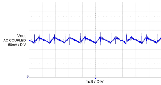
Output Ripple
