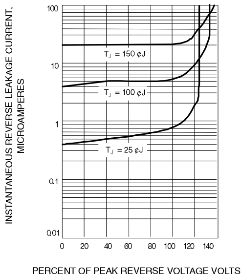
Fig. 3-TYPICAL REVERSE CHARACTERISTICS
