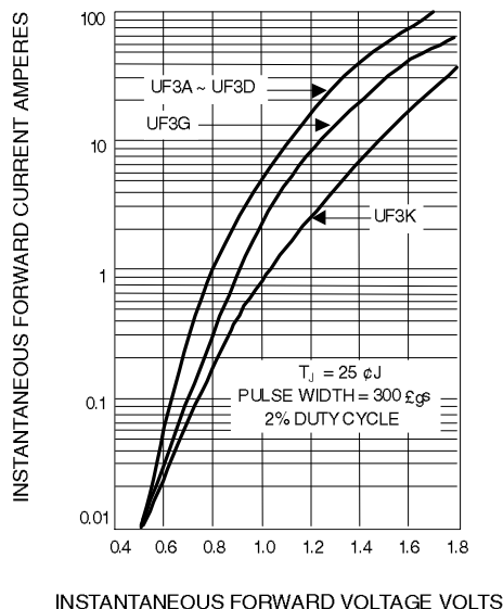
Fig. 4-TYPICAL FORWARD CHARACTERISTICS
