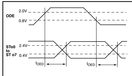
Figure 15 Output Driver Enable
