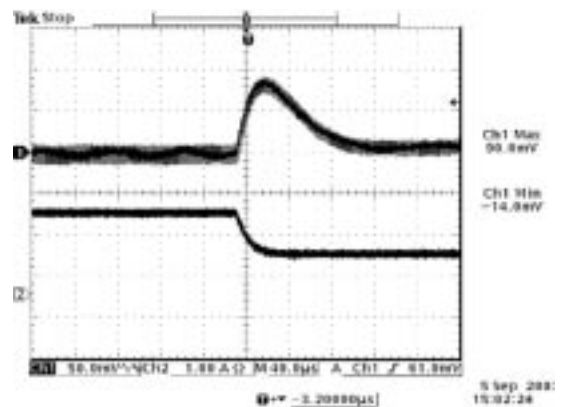
Vout=3.3V 100% to 50% load transients at 12V input and Ta=25° C
