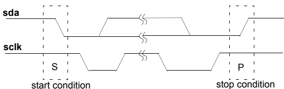
Figure 22. Start/Stop Conditions
