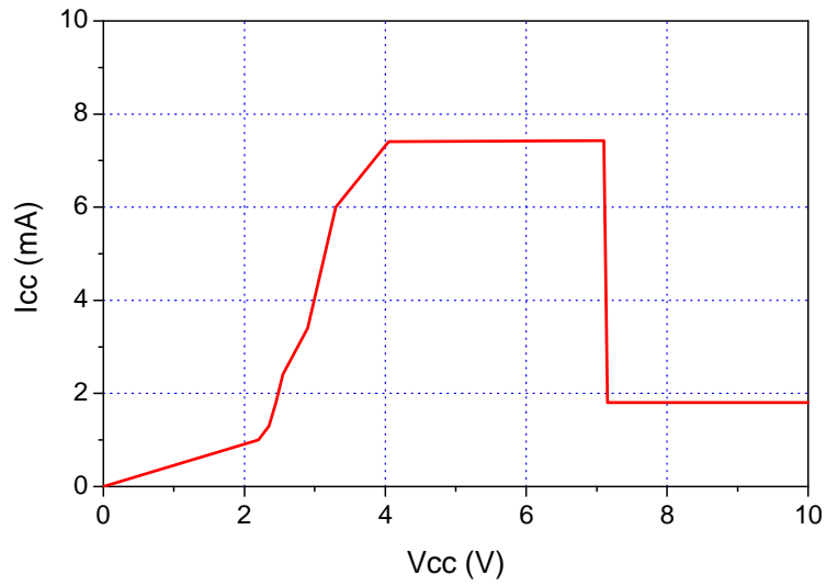
QUIESCENT CURRENT
