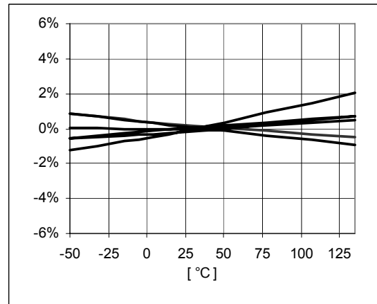
Fig. 7 Threshold Voltage Variation vs. Temperature (normalized)
