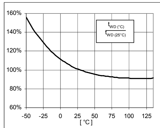
Fig. 9 Watchdog Timeout Period t_{WD} vs. Temperature (normalized with respect to t_{WD\ 25^\circ\text{C}} )
