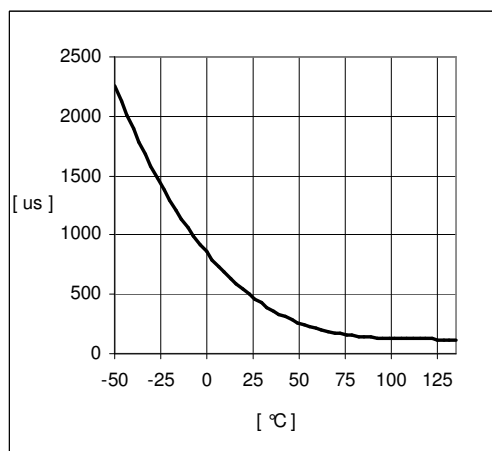
Reset Timeout Period t_{POR} vs. Temperature
