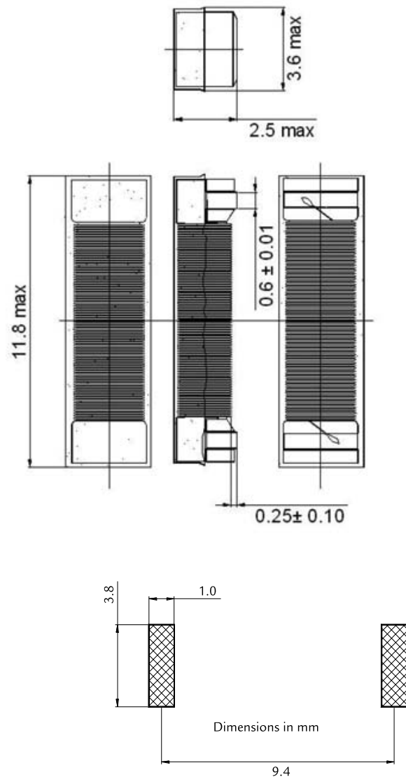
SDTR1103 DIMENSIONS AND RECOMMENDED LAYOUT
