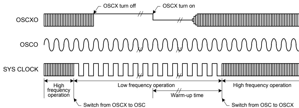
Timing of System Clock Switching
