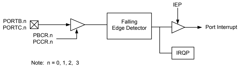
PORT Interrupt Block Diagram
