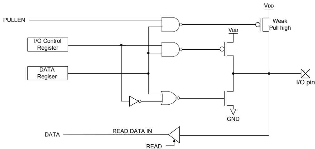
Port Configuration Function Block Diagram
