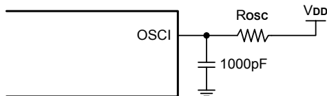
External RC
