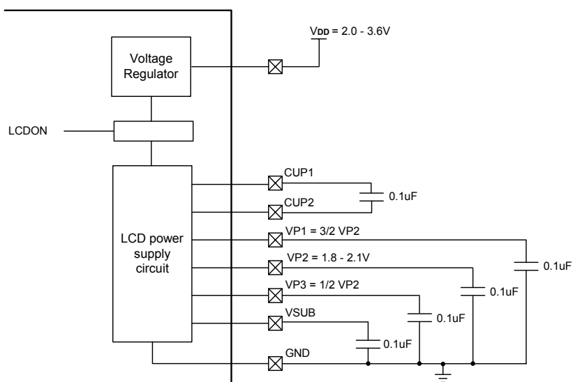
LCD Power Circuit Diagram
