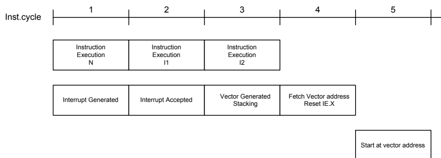
Interrupt Servicing Sequence Diagram
