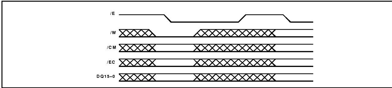
Figure 4: Write Cycle
