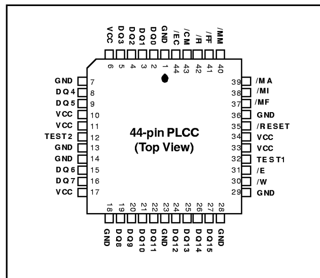
PINOUT DIAGRAM
